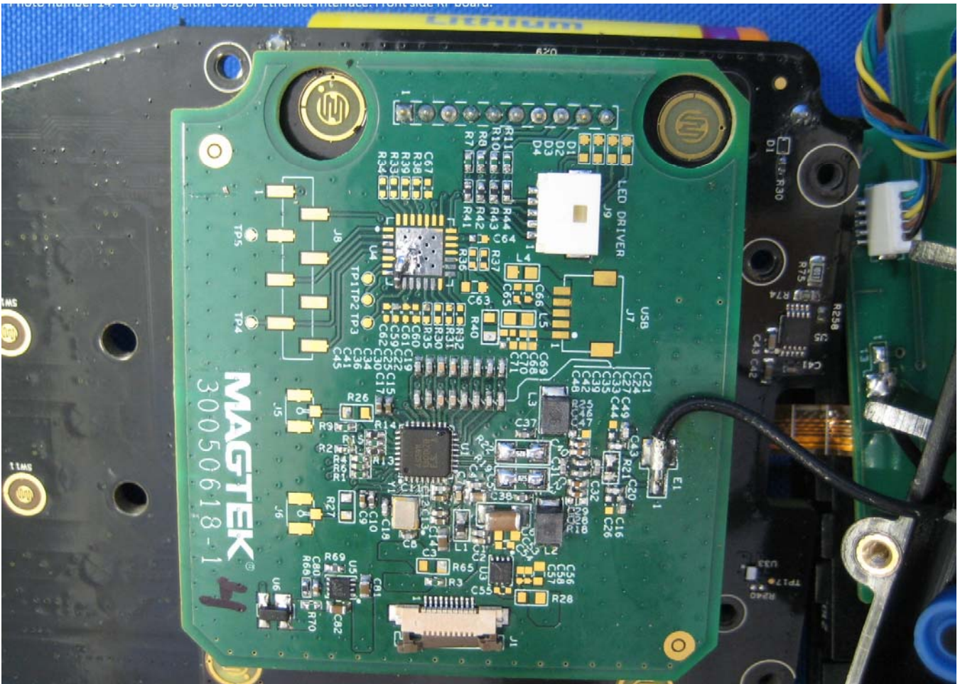
Photo number 14. EUT using either USB or Ethernet interface. Front side RF board.
