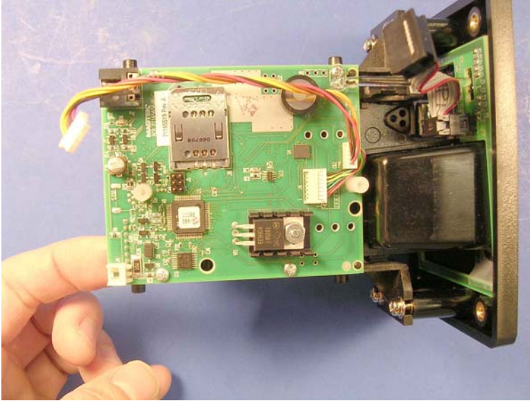
Logic PCB
