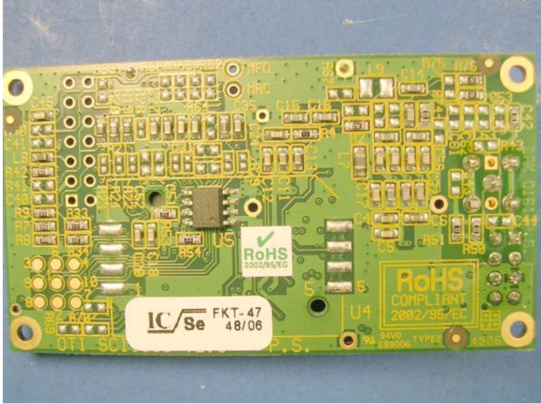
Transmitter PCB Bottom
