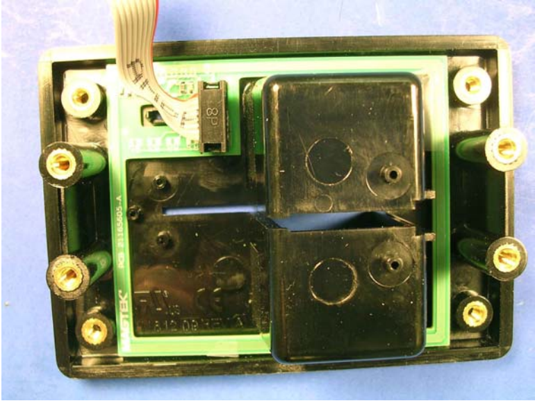
Antenna 1
