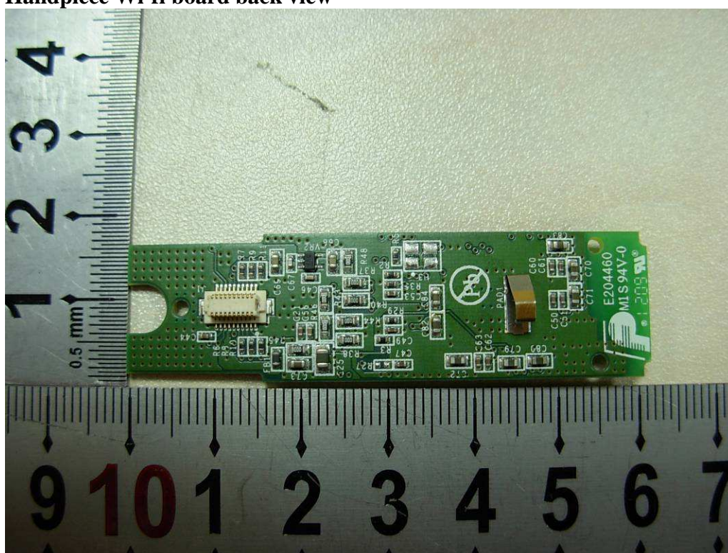
Handpiece Wi-fi board back view
