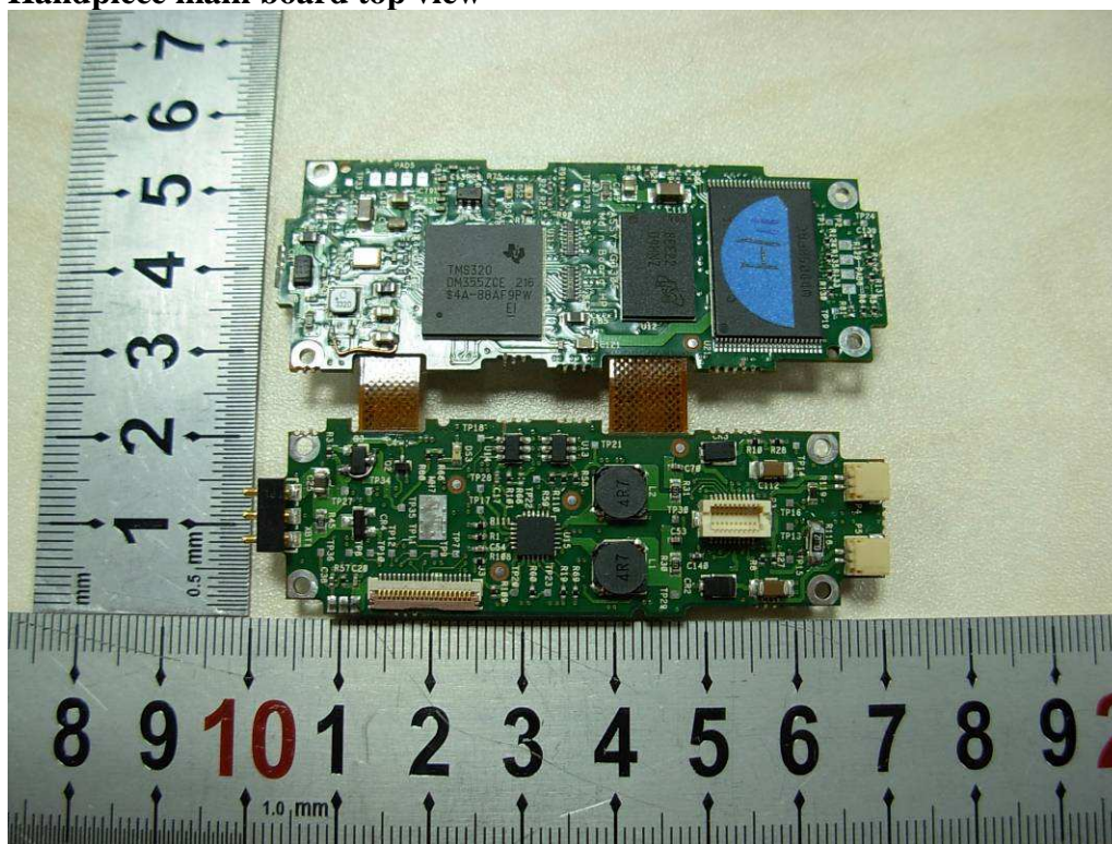
Handpiece main board top view
