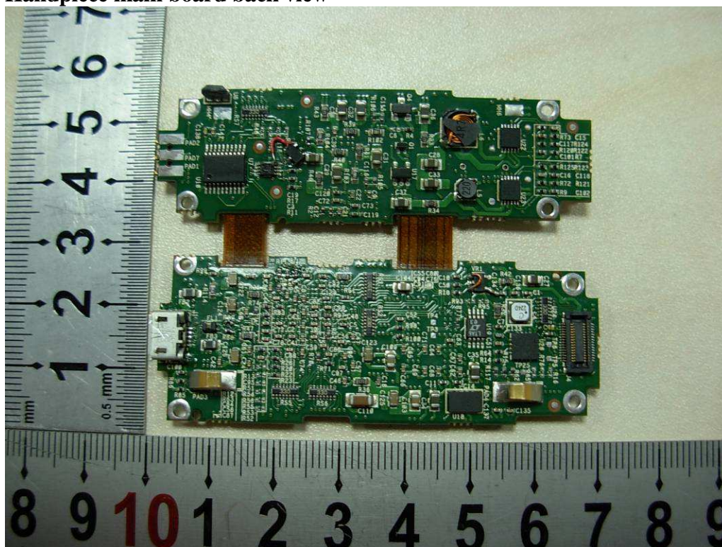
Handpiece main board back view
