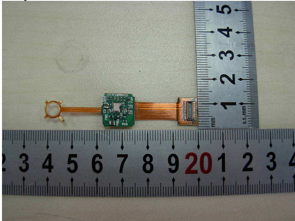
Handpiece Sensor board
