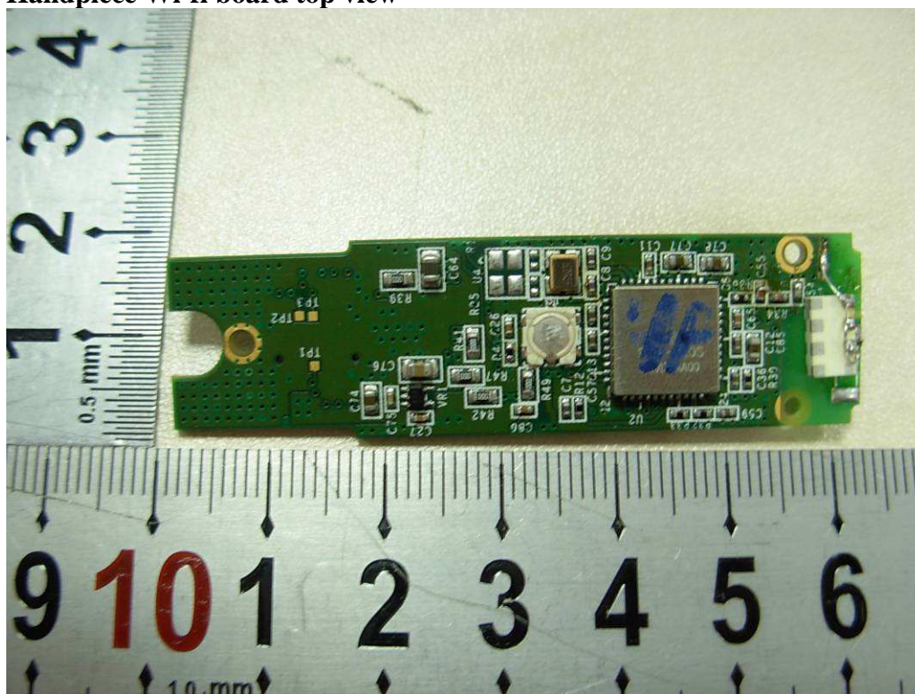
Handpiece Wi-fi board top view
