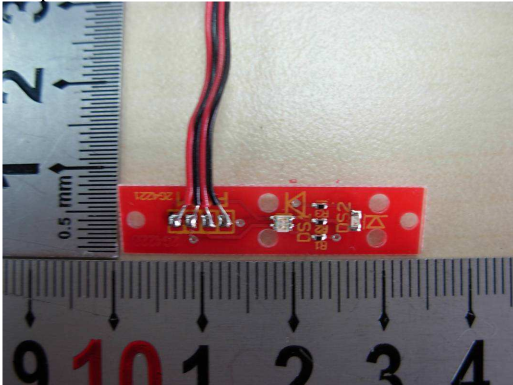
Handpiece LED board
