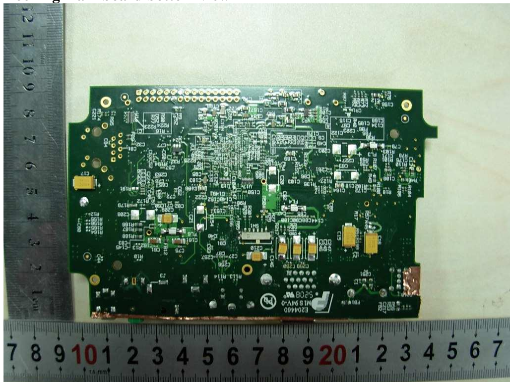
Docking main board bottom view
