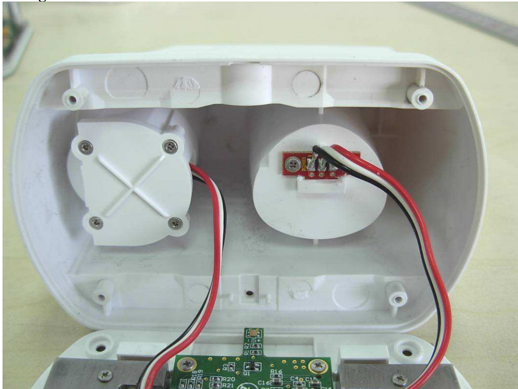
Charger internal view
