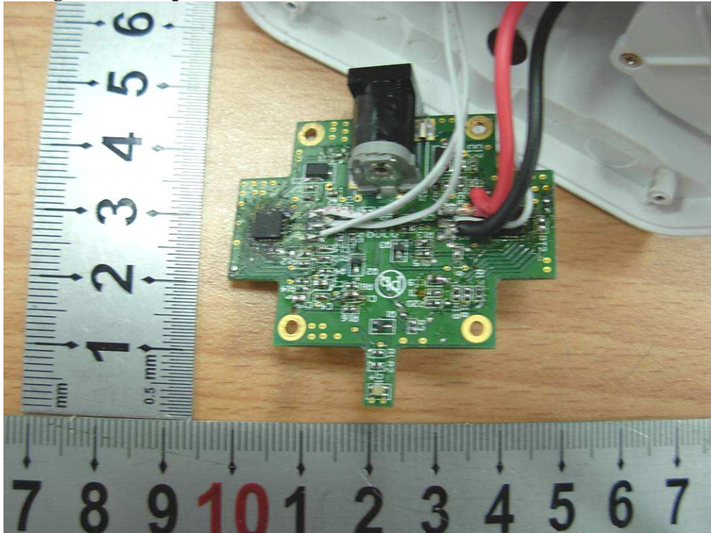
Charger Board top view
