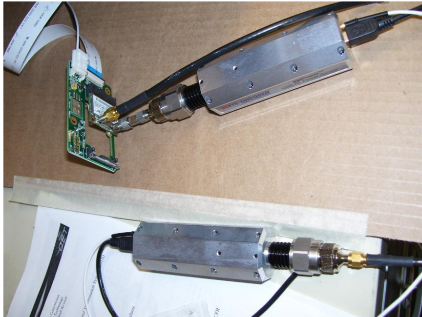
Figure 1: Conducted Measurements from antenna port(s)
