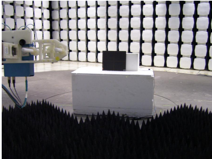
Figure 3: Radiated Measurements for C63.10:2009
