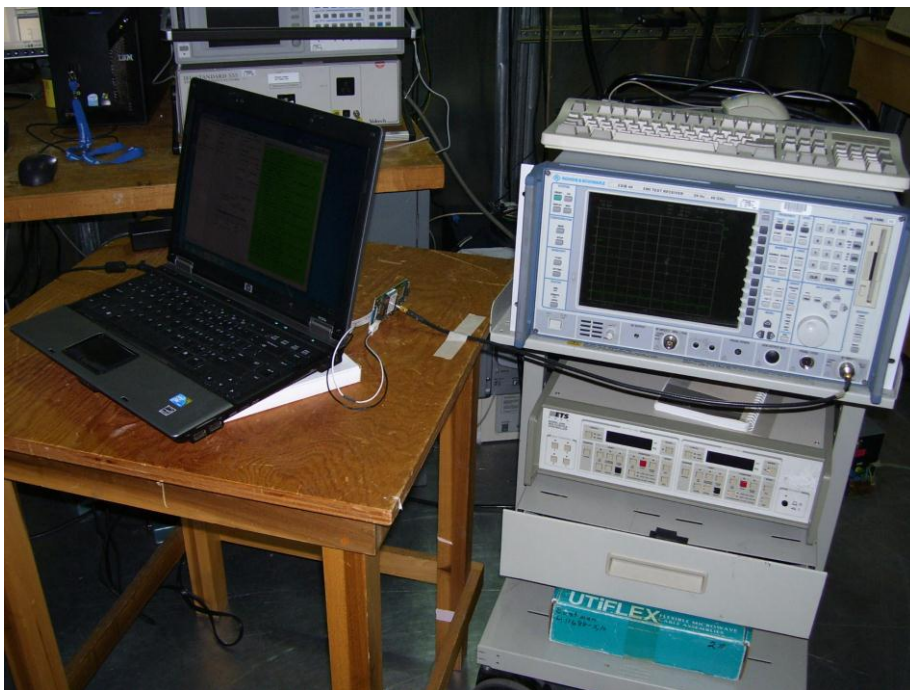
Figure 2: Conducted Measurements from antenna port(s)
