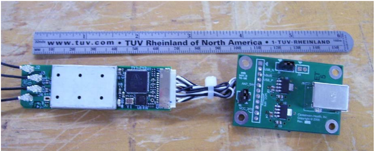
Figure 1 – Radio and interface device used for testing (front)
