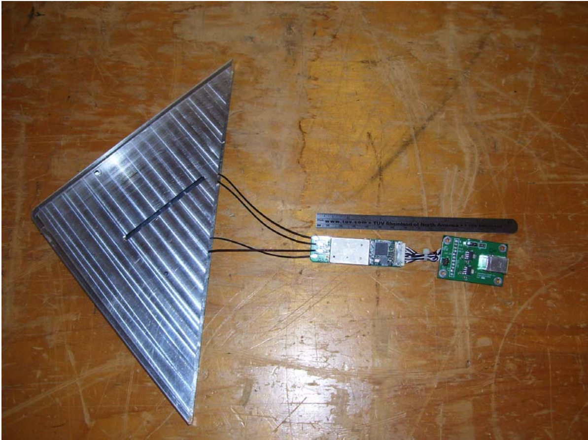
Figure 3 – Radio attached to partial enclosure with antenna's installed
