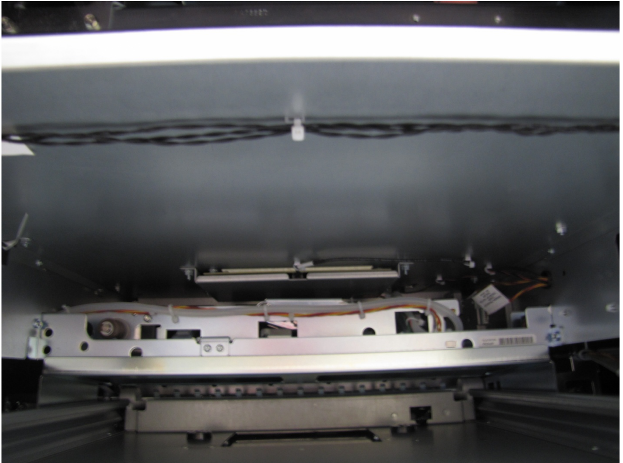
RF Tag Antenna Inside DRYVIEW 5950 Bottom View
