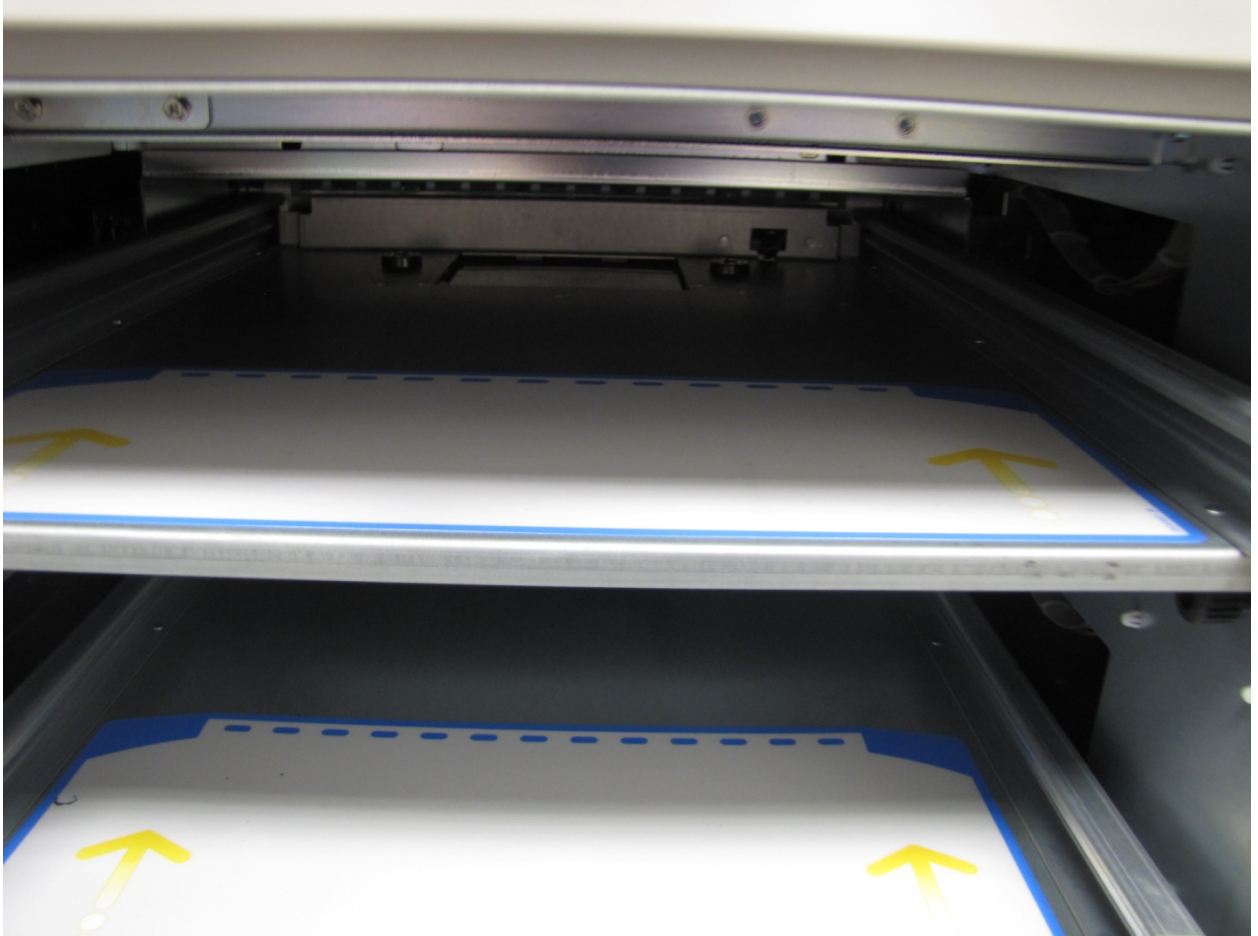
RF Tag Antenna Inside DRYVIEW 5950 Top View
