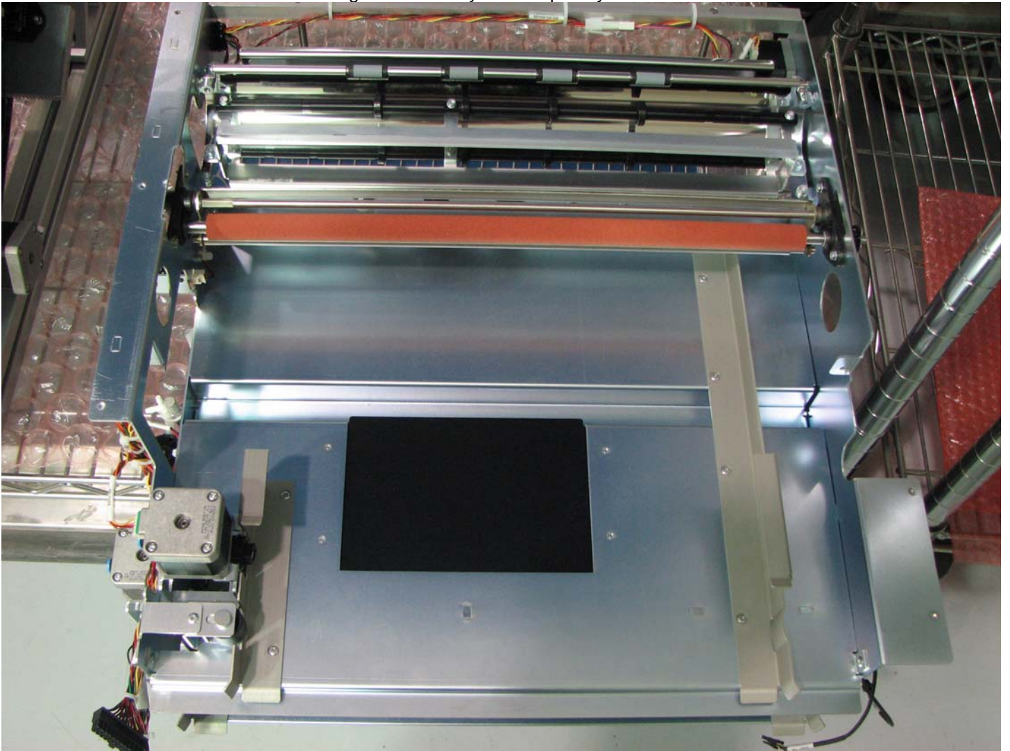
RF Tag Antenna Assy-In Pickup Assy-from above
