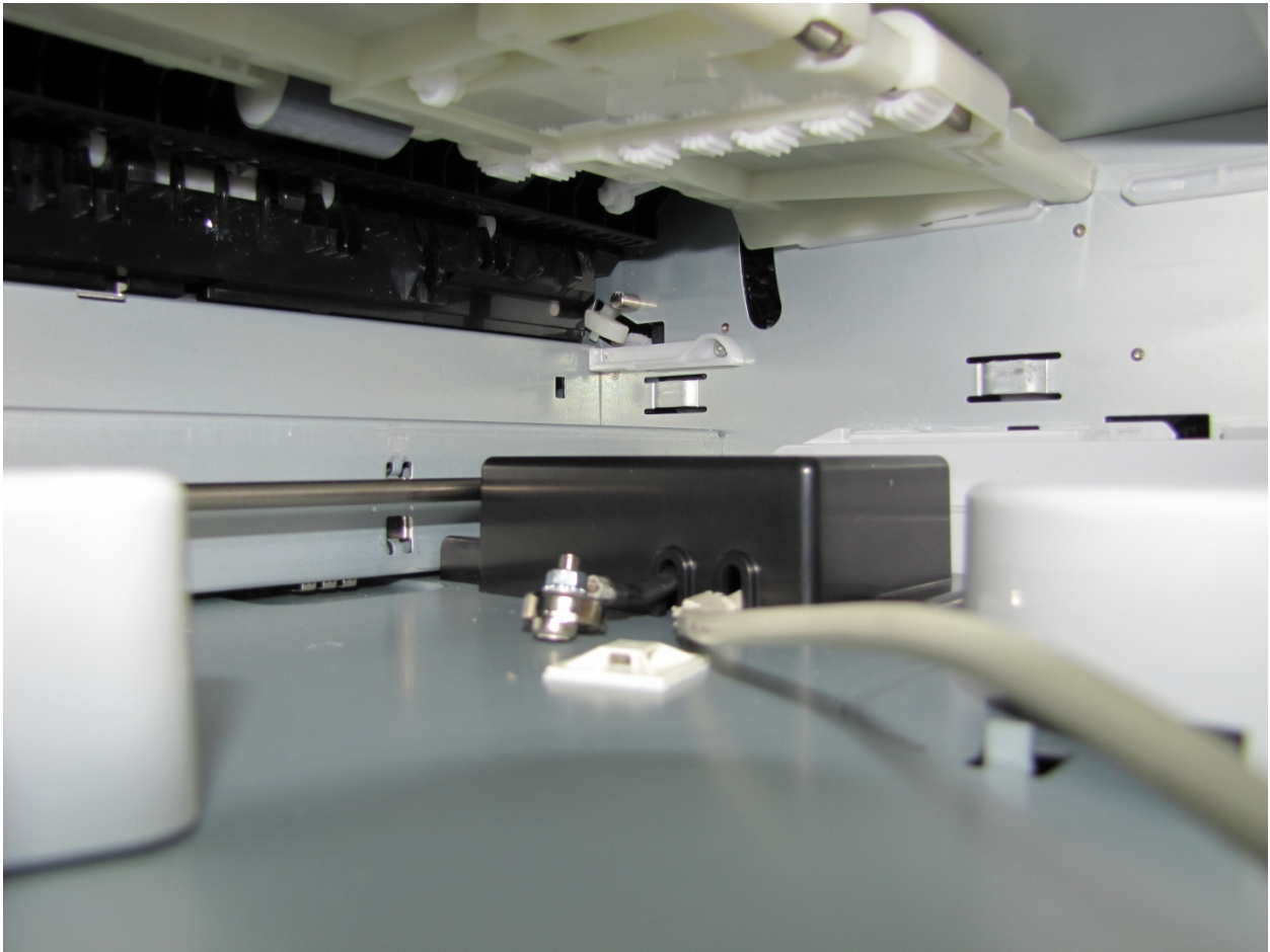
RF-Tag Dual Antenna Board Enclosure - Inside Imager – Side View
