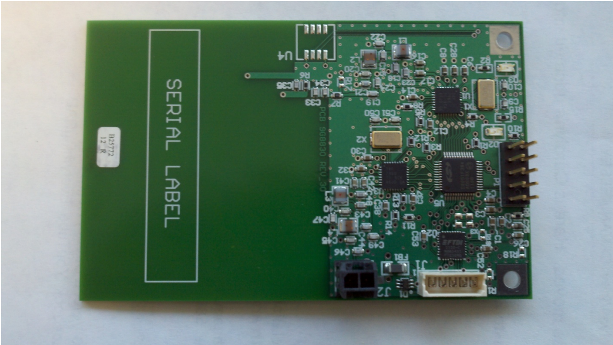
RF-Tag Dual Antenna Board - Component Side
