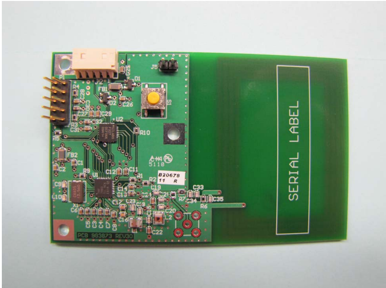
Chroma RF-Tag Board Components Side
