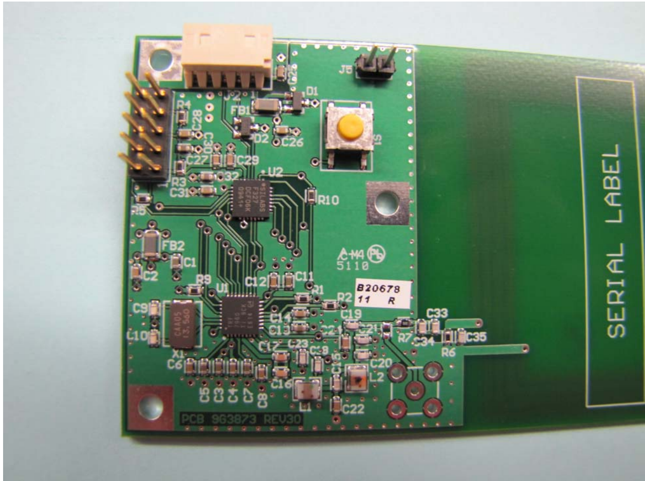
Chroma RF-Tag Board Components Side – Closer View
