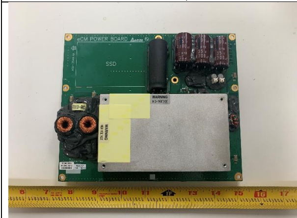
EUT-PCBA2-Top
