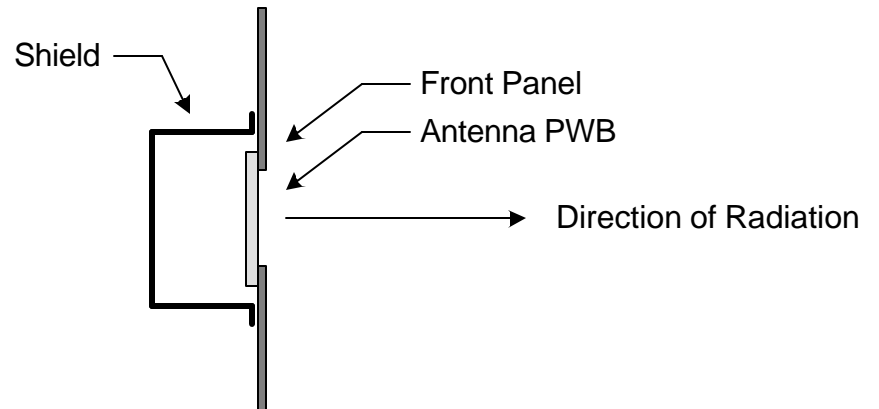
Antenna Detail Side View
