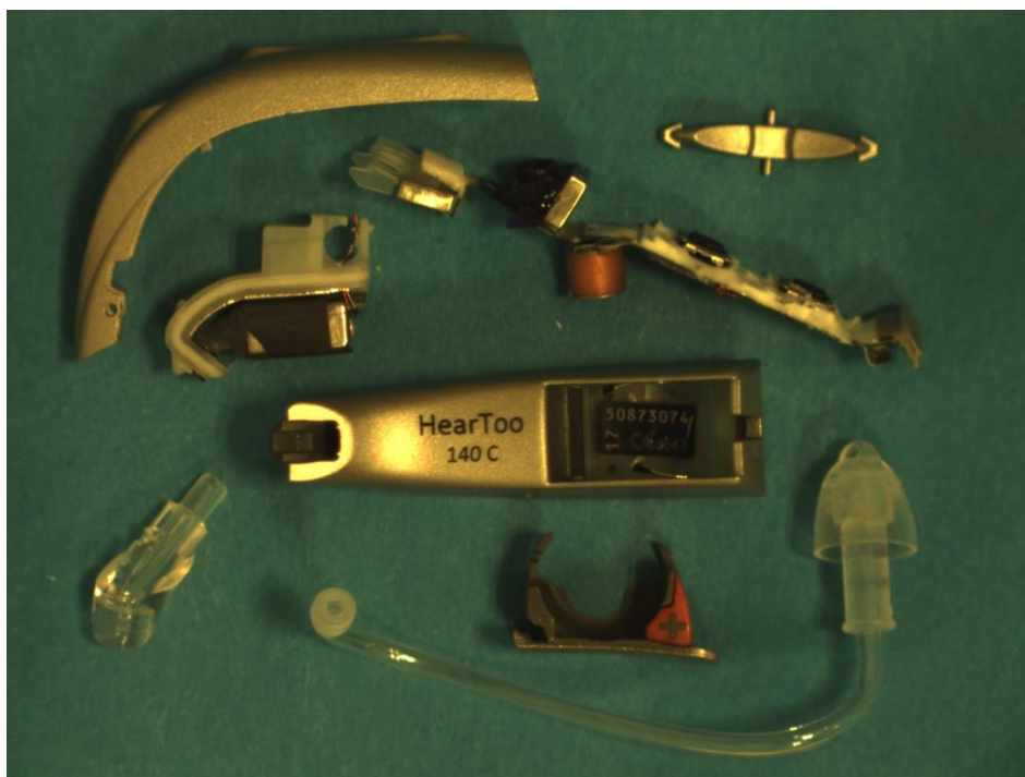
Photo of exploded parts of HearToo 140 C
