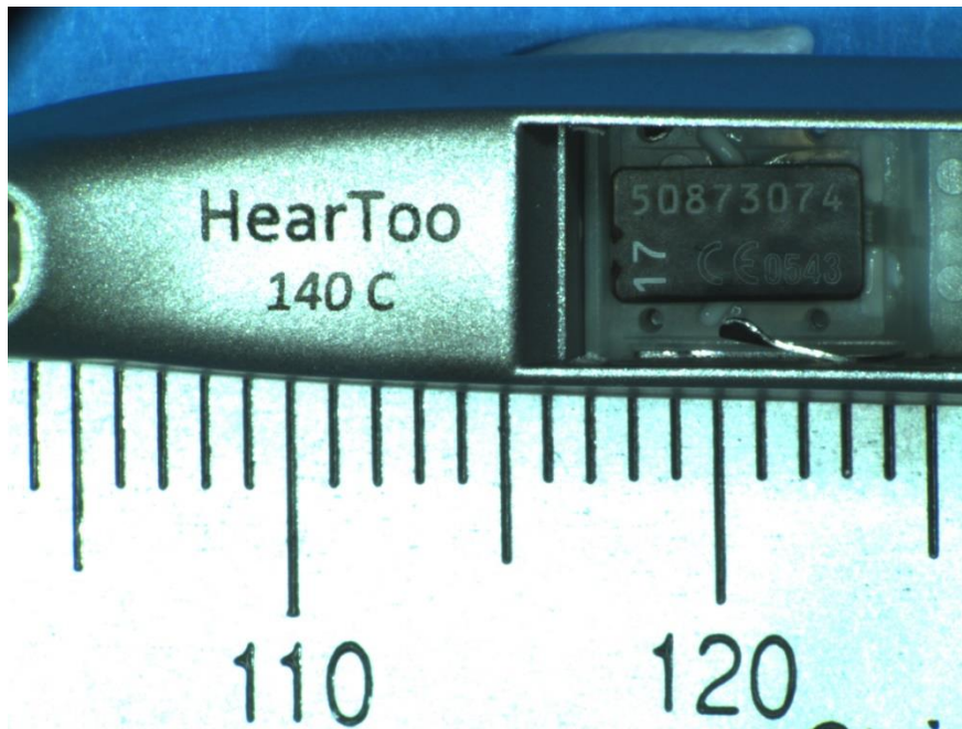
Photo of Labels inside and outside HearToo 140 C
