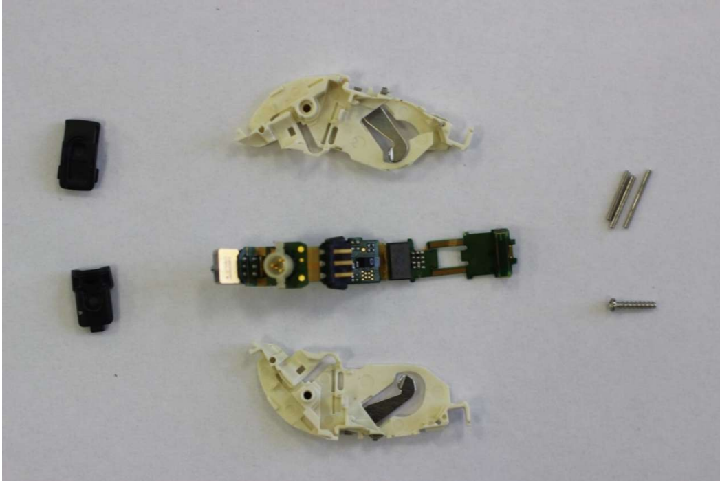
PCB showing the connector side
