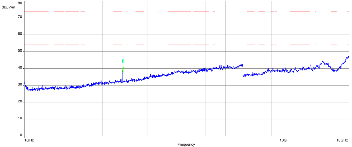
Plot 1: 1 GHz to 18 GHz, RX / idle – mode, lowest channel, vertical & horizontal polarization
