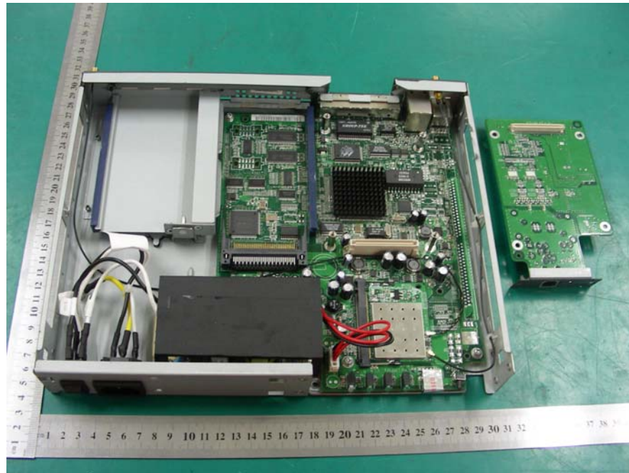
H3C MSR 20-13; Quidway AR 19-13 Internal view (2)
