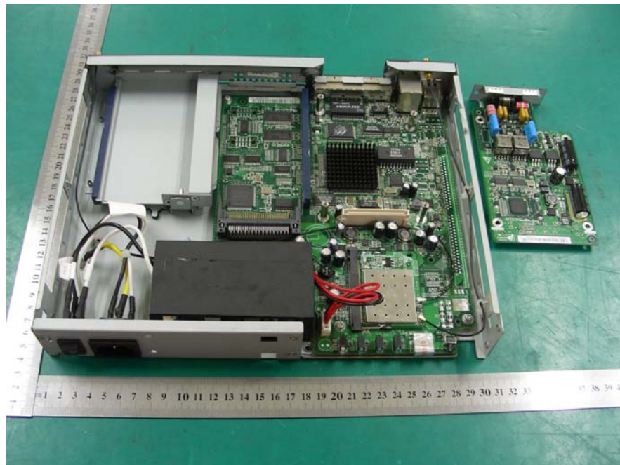
H3C MSR 20-13; Quidway AR 19-13 Internal view (1)
