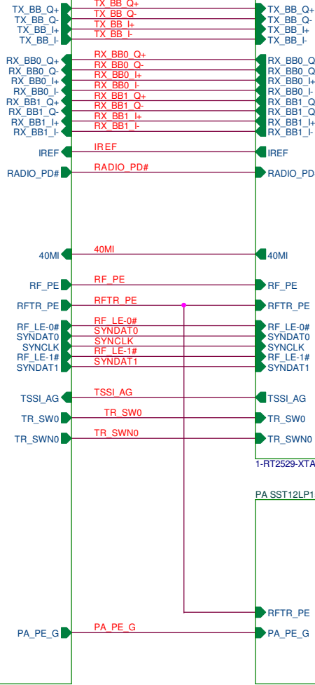
2-PA-SST12LP15A-LNA
