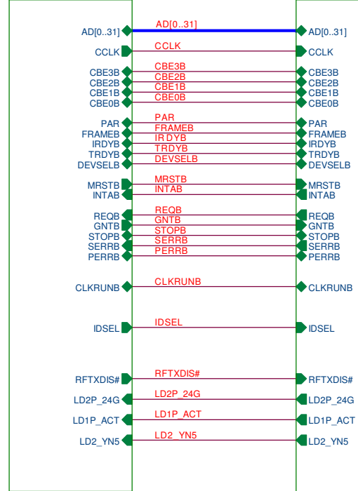
4-MINIPCI.SCH
