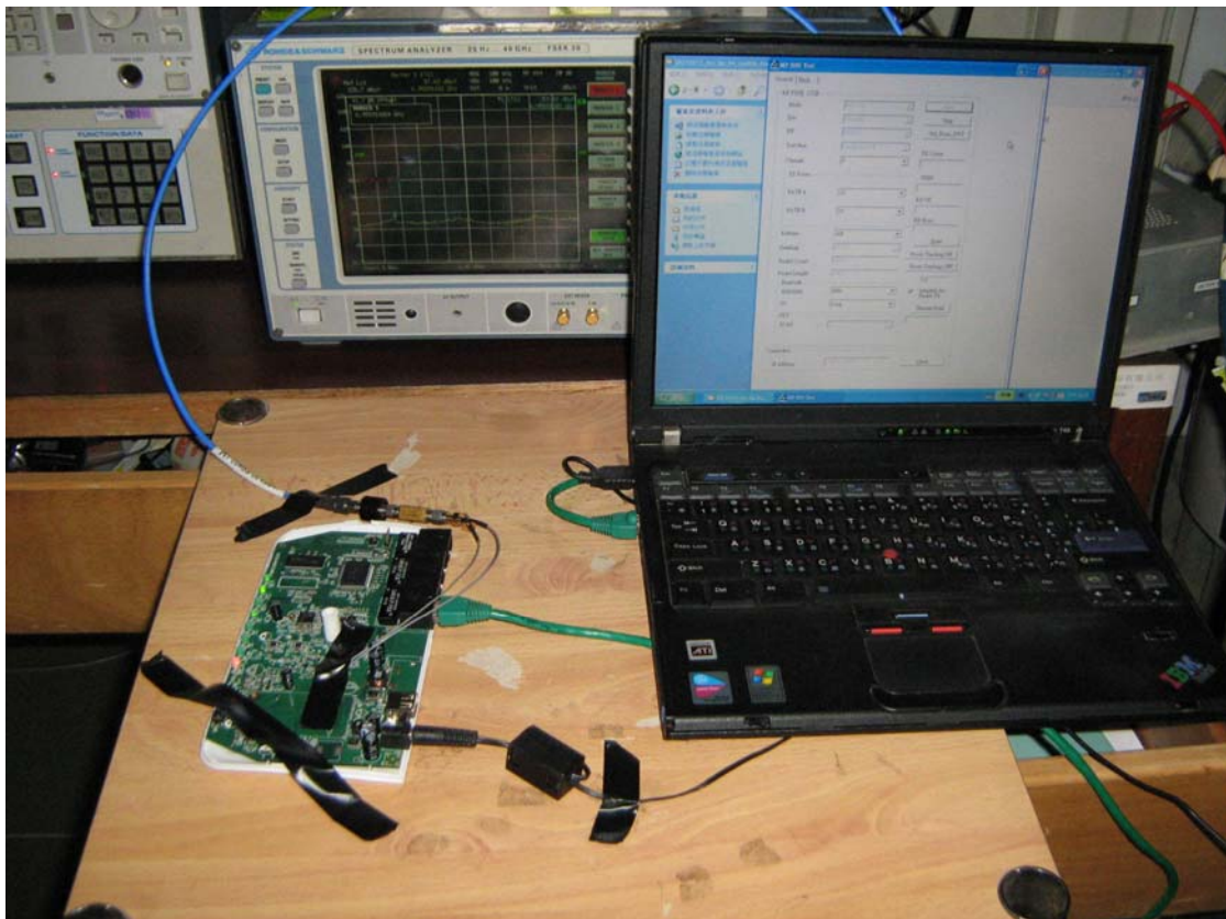
CONDUCTED EMISSIONS MEASUREMENT SETUP
