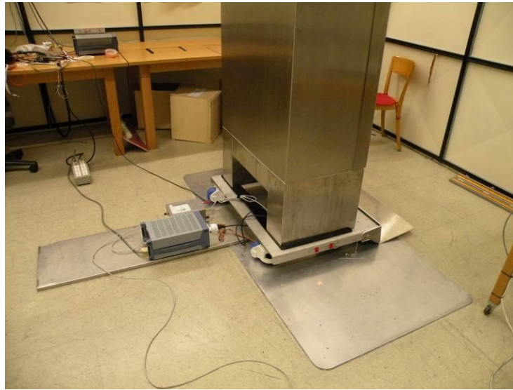
Photo 1: Conducted disturbances
