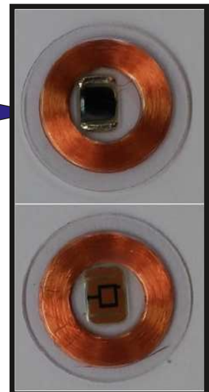
Passive TAG (HID to 125Khz)
