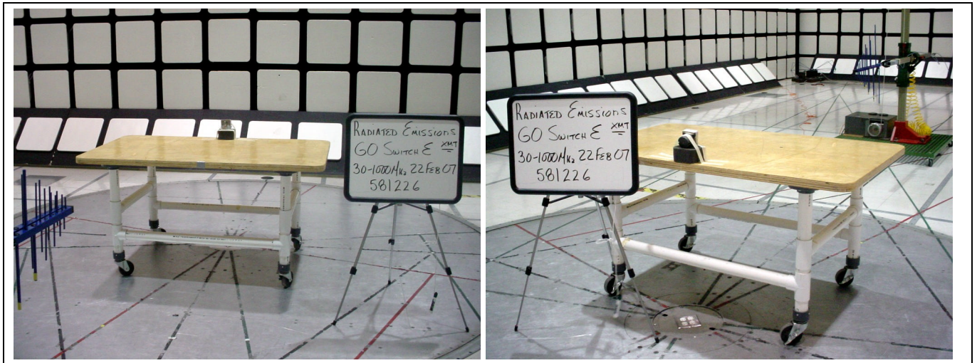
Figure 15 Test setup for Radiated Emissions –30MHz-100MHz
