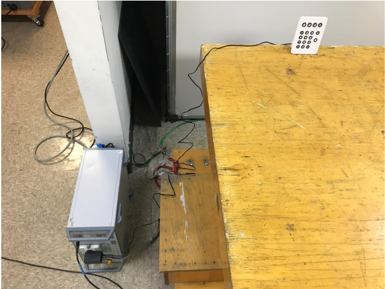
Photograph 4: AC Line Conducted
