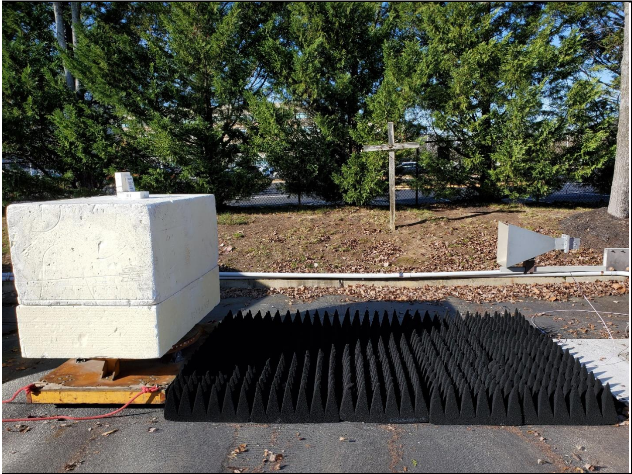
Photograph 3: Radiated Testing – Side View of Testing Over 1 GHz
