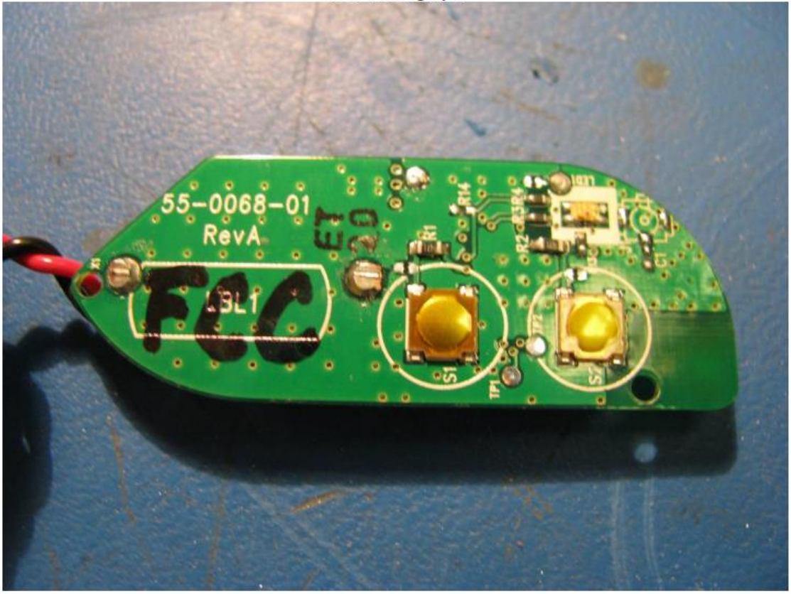
EUT Photograph
