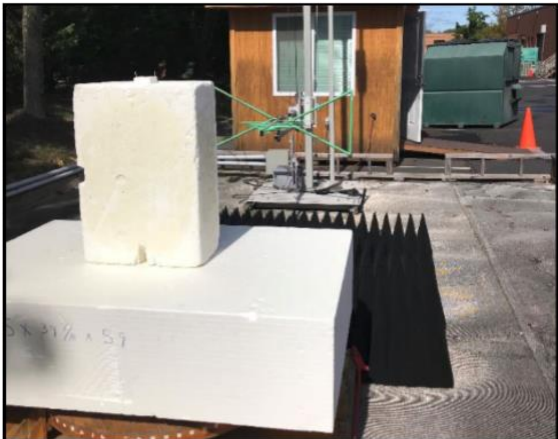
Radiated Emissions (Greater Than 1GHz)
