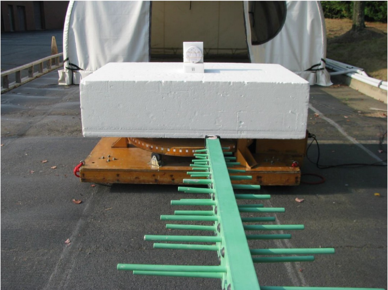
Radiated Emissions
