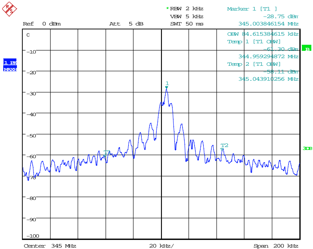
Plot: OBW 99%
