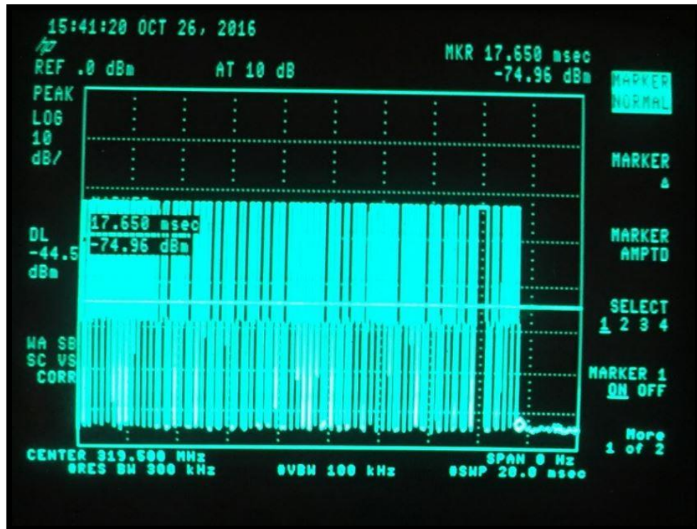
Figure 2: Packet Width
