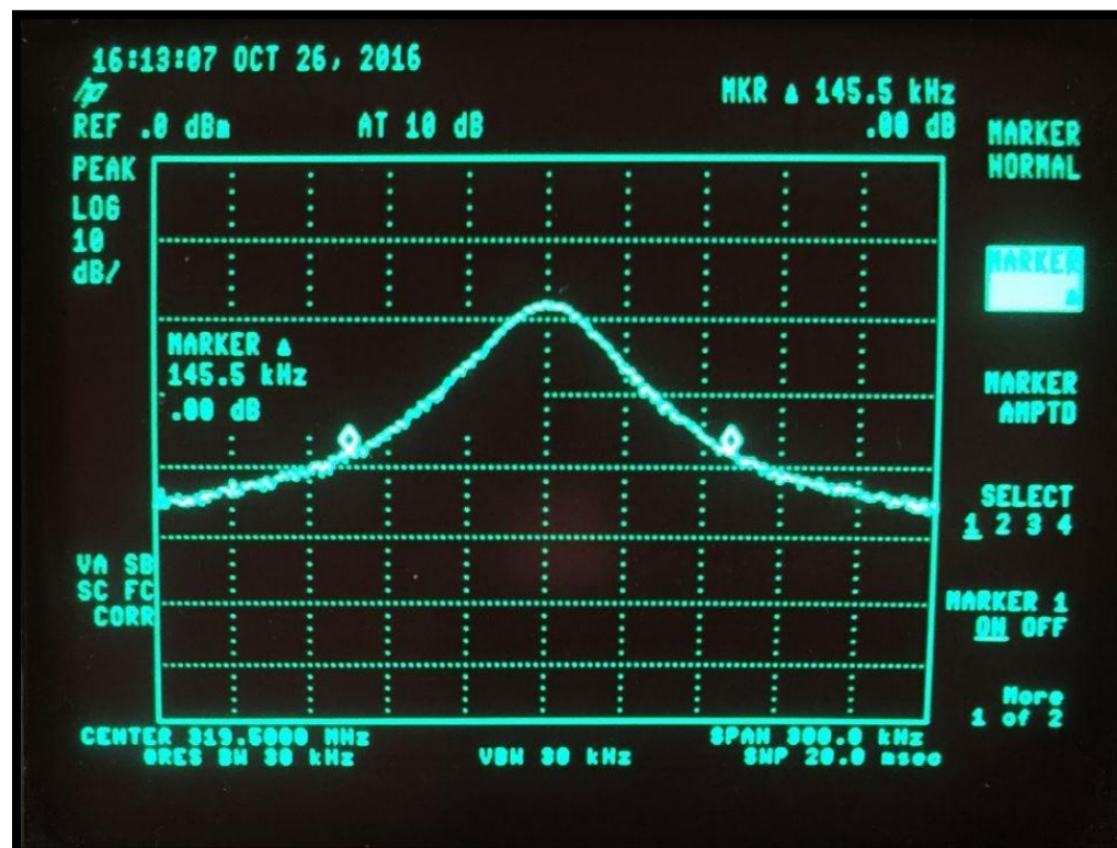
Figure 3: Measured Bandwidth
