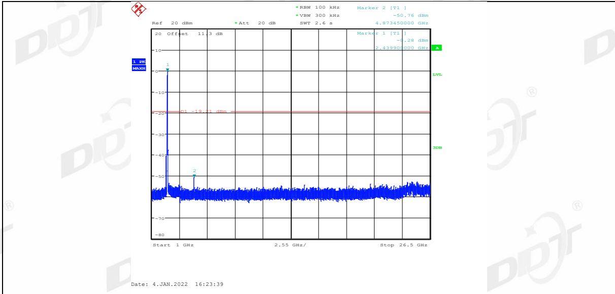
11N40SISO_Ant1_2452_0~Reference
