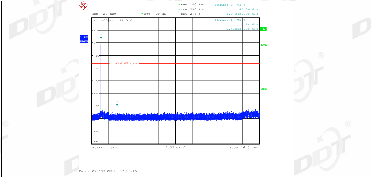
11N20SISO_Ant1_2462_0~Reference
