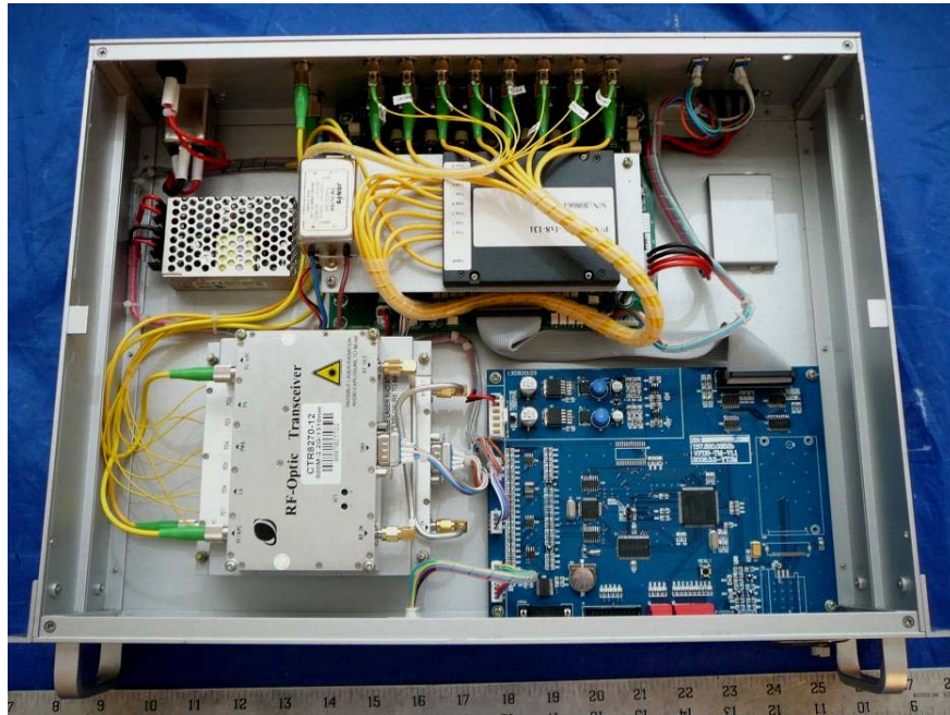
E-HUB Cover off View
