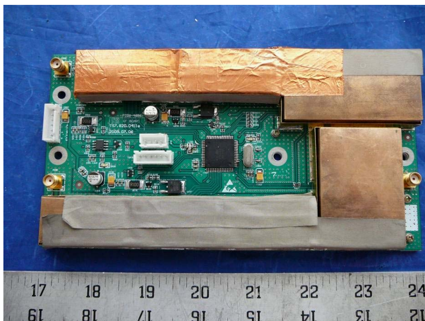
EUT RF Board Top View (With Shielding on) – RUB
