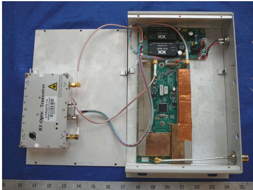
EUT Cover off View - RUB
