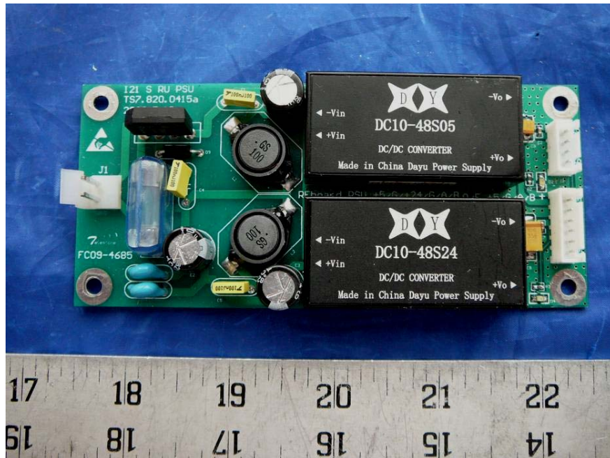
EUT Power Board Top View – RUB
