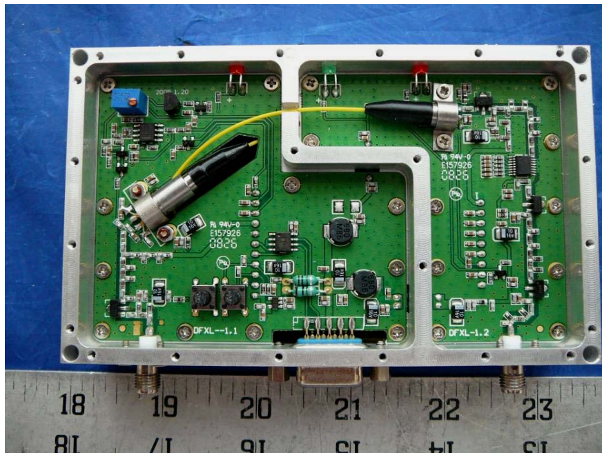
RF-Optical Transceiver Cover off View (2)
