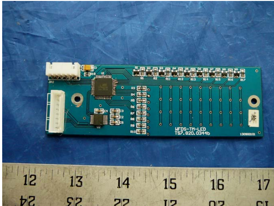
E-HUB LED Board Top View
