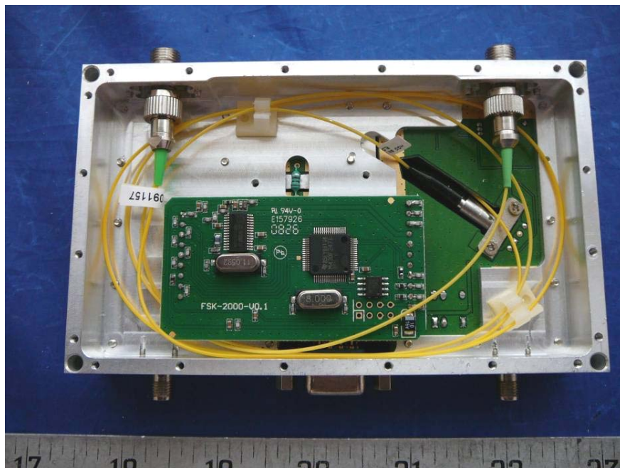
RF-Optical Transceiver Cover off View (1)
