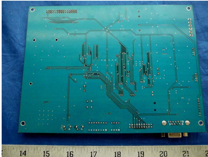
M-HUB Main PCB Board Bottom View
