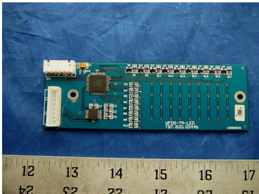
M-HUB LED Board Top View
