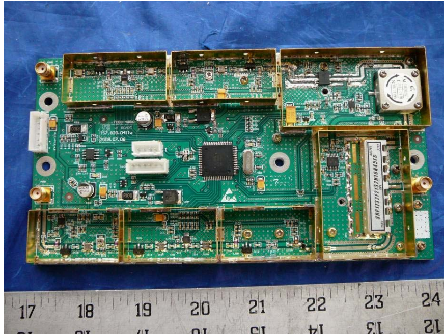
EUT RF Board Top View (With Shielding off) – RUB
