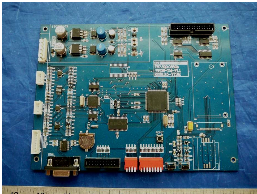
E-HUB Main PCB Board Top View
