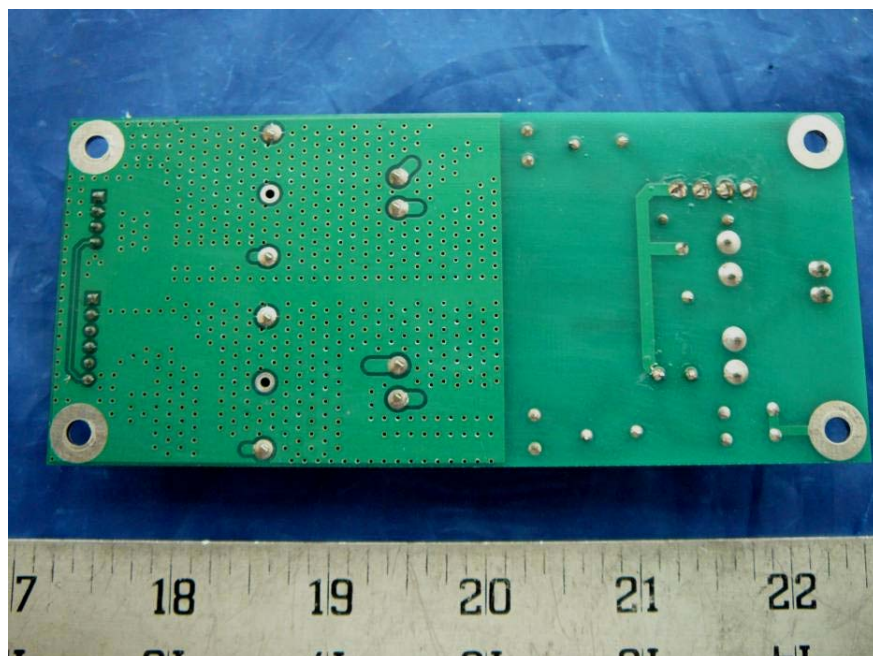
EUT Power Board Bottom View – RUB
