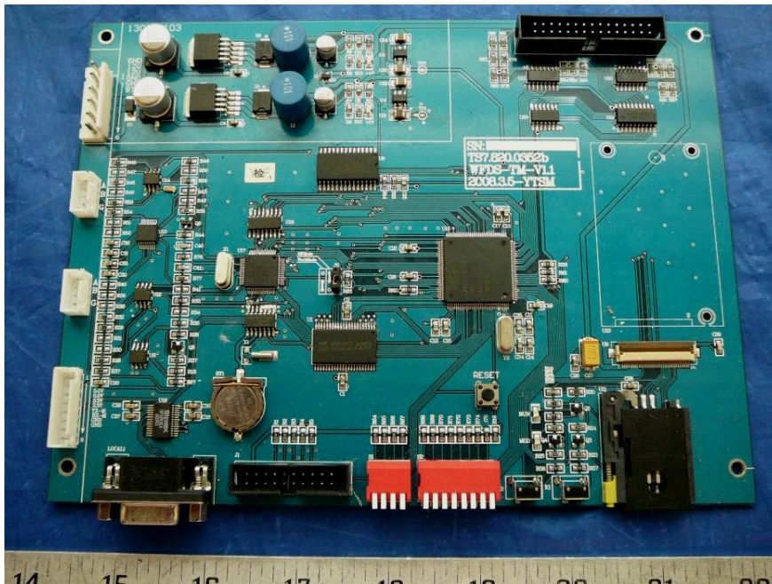
M-HUB Main PCB Board Top View
