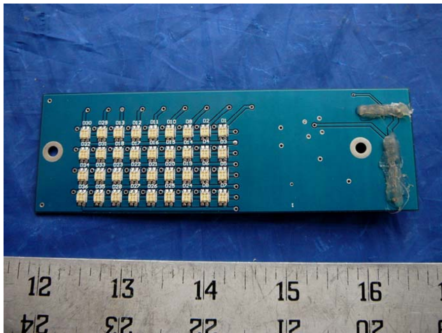
E-HUB LED Board Bottom View
