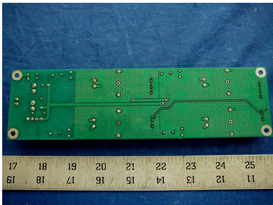
EUT Power Board Bottom View – RUA
