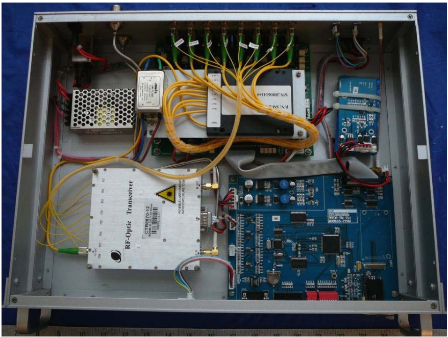
M-HUB Cover off View
