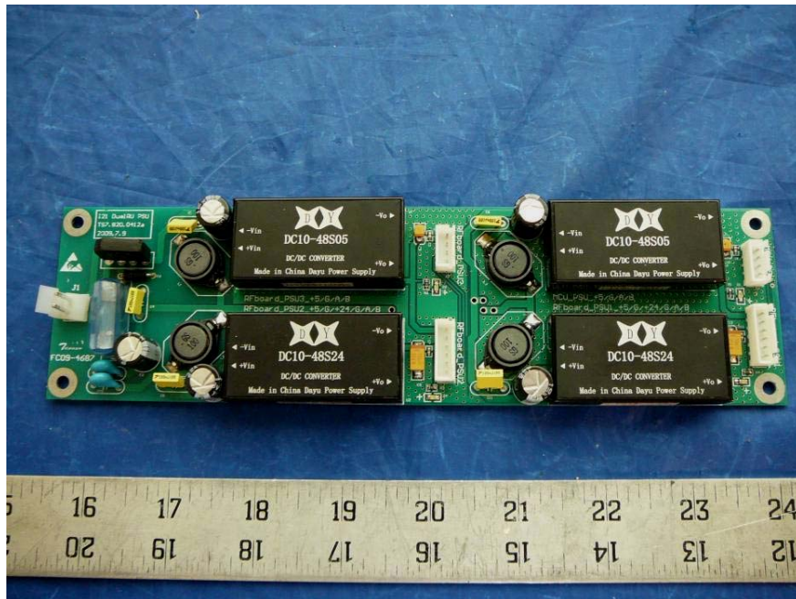
EUT Power Board Top View – RUA
