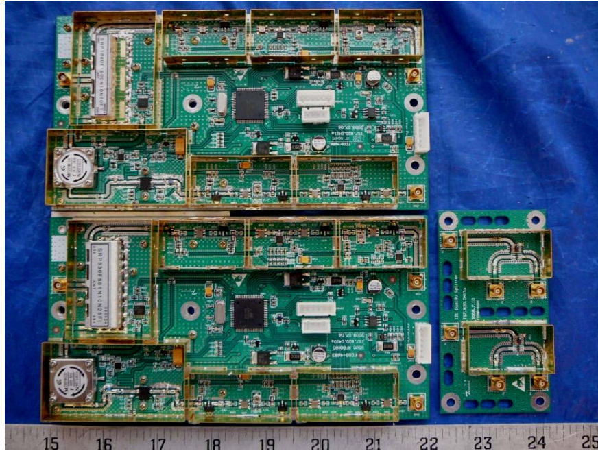
EUT RF Board Top View (With Shielding off) – RUA
