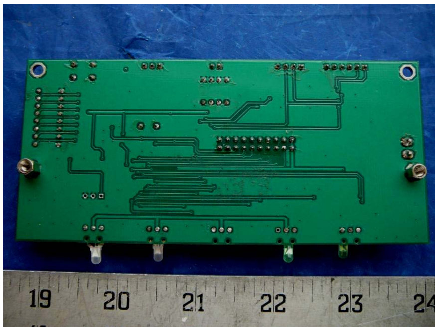
EUT LED Board Bottom View – RUA
