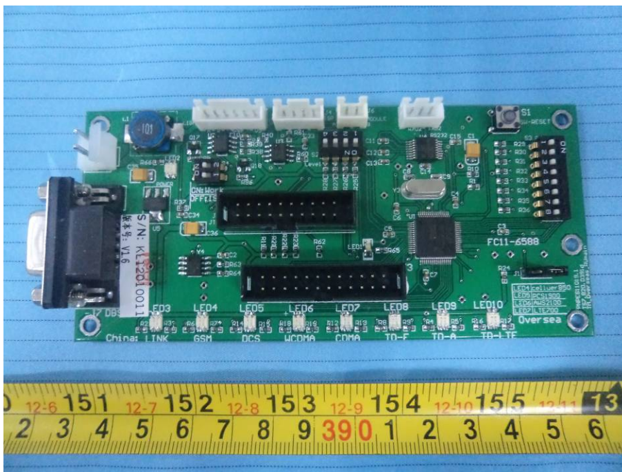
EUT – Remote Unit Debug Board Top View
