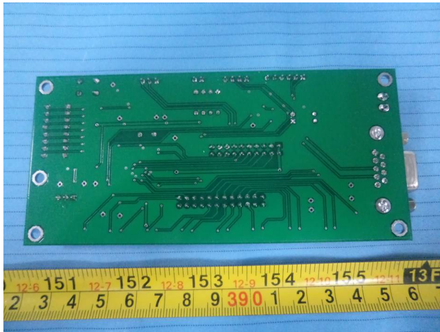
EUT – Remote Unit Debug Board Bottom View
