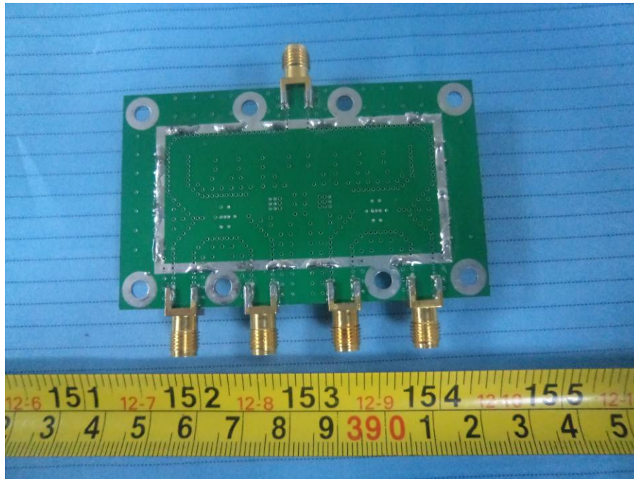
EUT – Remote Unit RF Splitter Board 2 Bottom View
