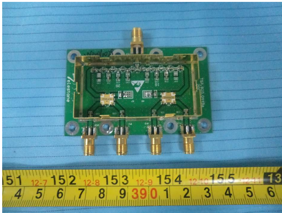
EUT – Remote Unit RF Splitter Board 2 Top Shielding off View
