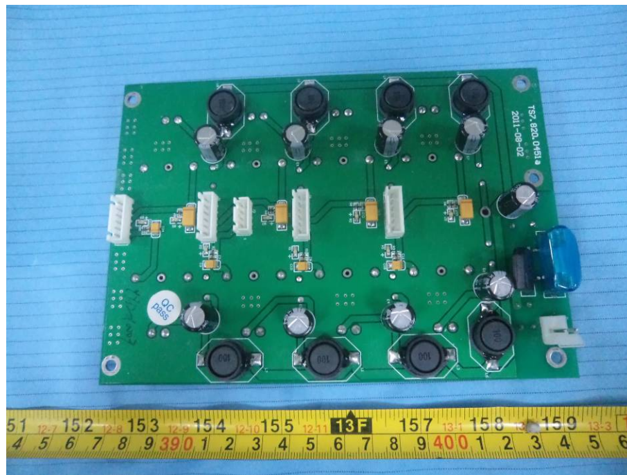
EUT – Remote Unit CEC Board Bottom View
