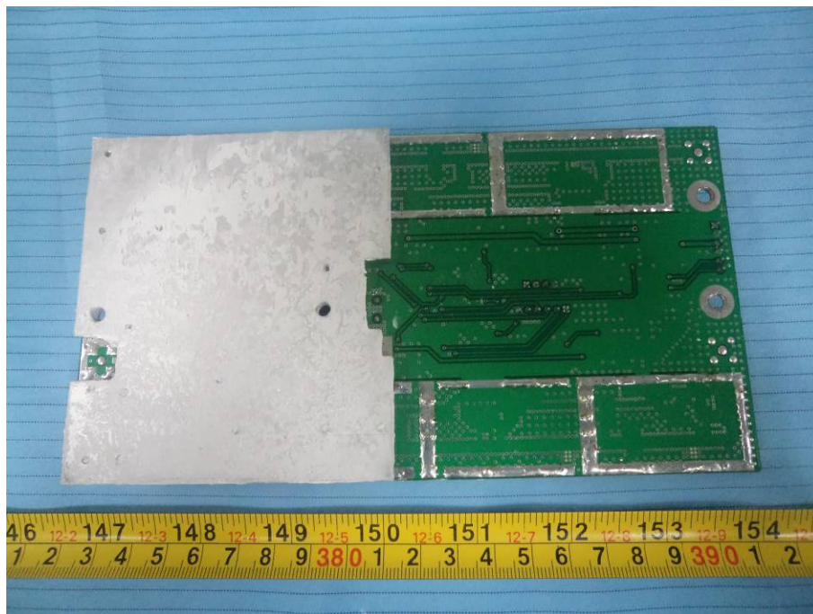
EUT – Remote Unit RAU-Cellular-881-21 Board Bottom View 1
