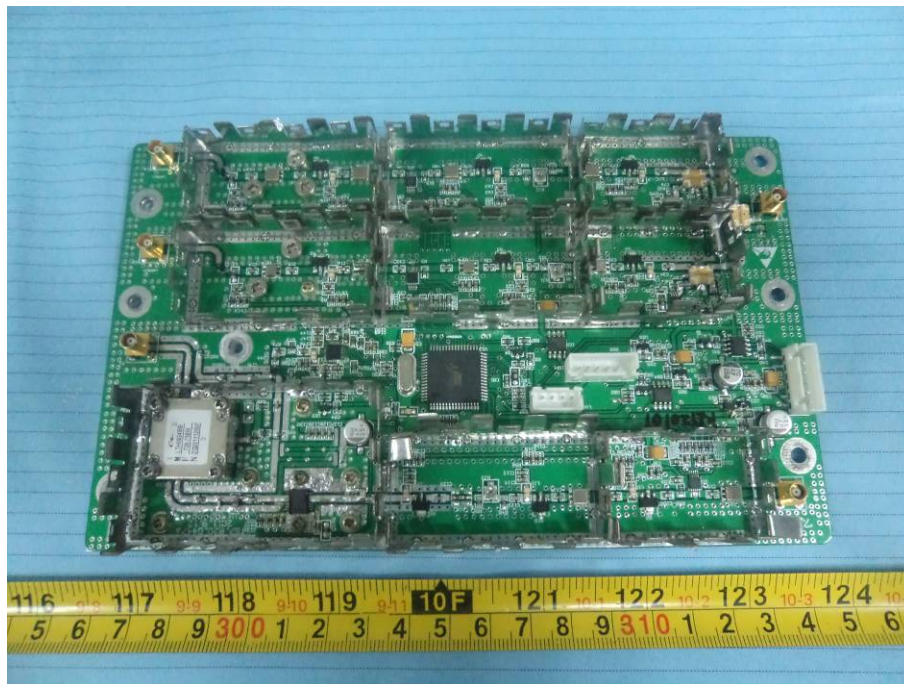
EUT – Remote Unit LTE700 Board Top Shielding off View
