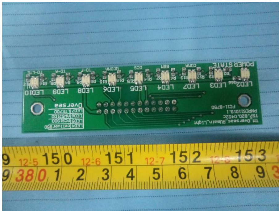
EUT – Remote Unit LED Board Top View
