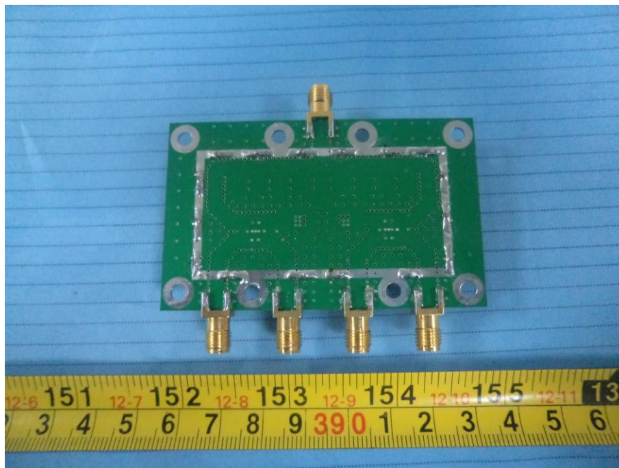
EUT – Remote Unit RF Splitter Board 1 Bottom View
