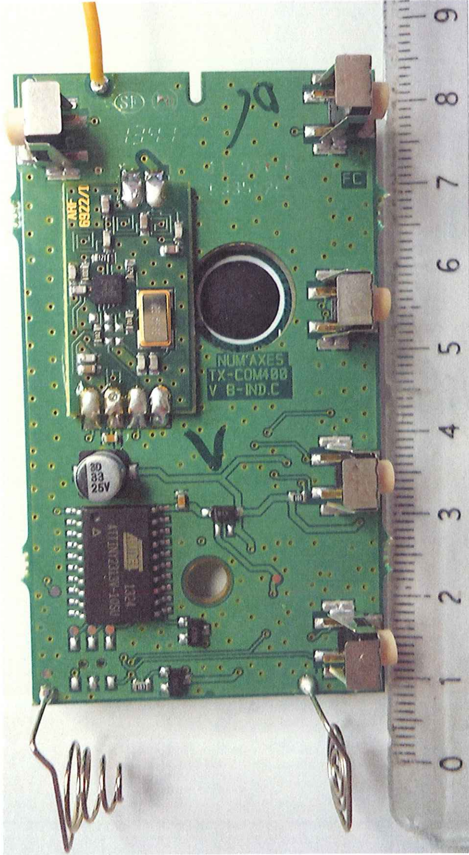
450 Transmitter_IntPho.pdf : interior photos of the equipment
