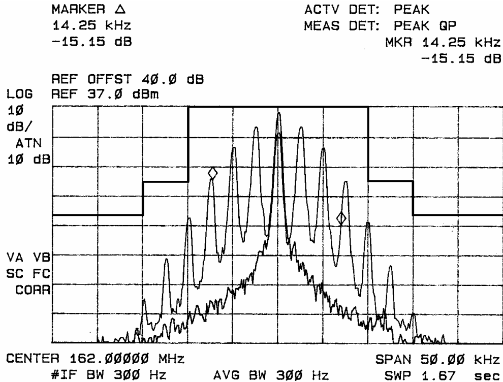
Figure five Occupied Band Width, wide band, no squelch tone
