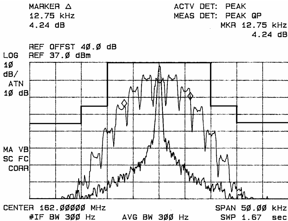
Figure six Occupied Band Width, wide band, CTCSS
