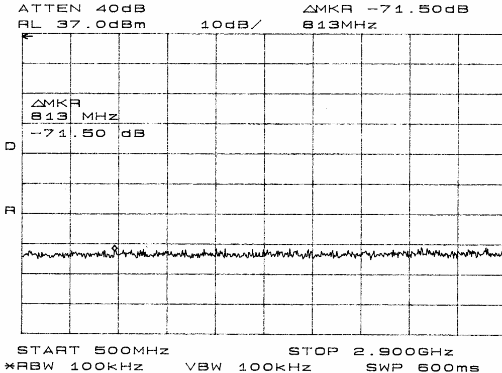
Figure twelve Emissions at Antenna Terminal (5 watt)
