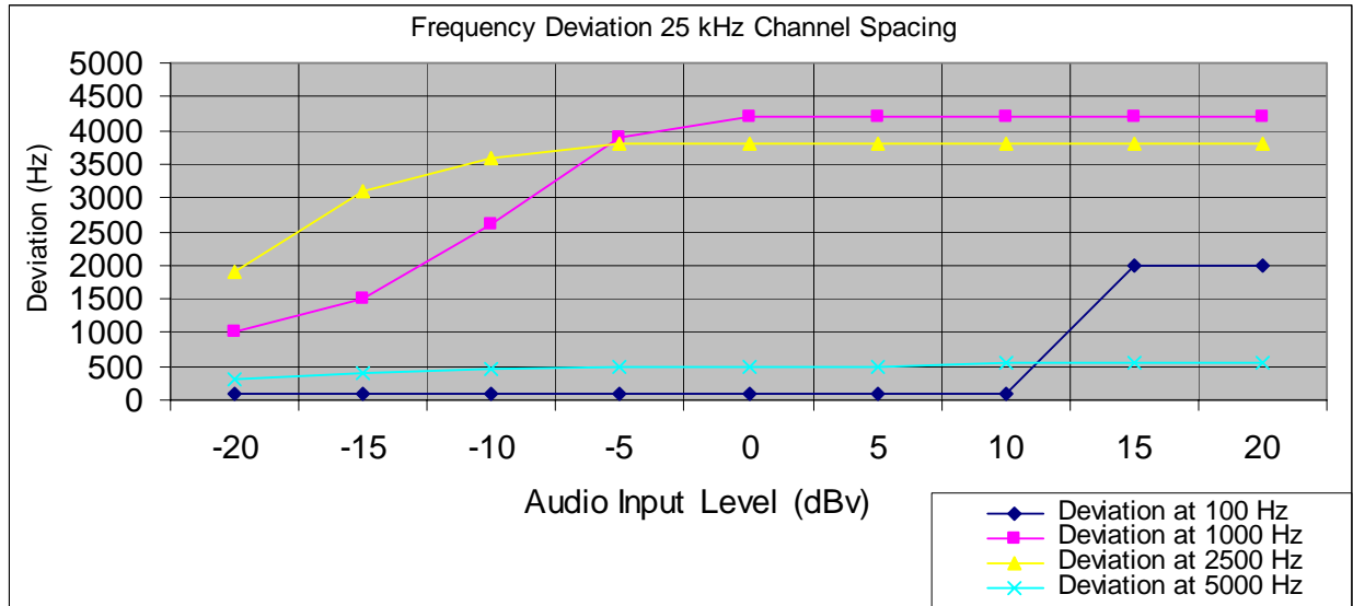
Figure two Frequency Deviation Characteristics (25 kHz Channel spacing)
