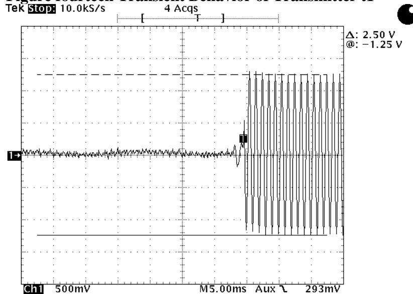
Figure fourteen Transient Behavior of Transmitter t1
