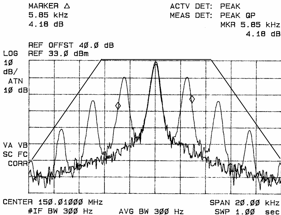
Figure eight Occupied Band Width, Narrow band, no squelch tone
