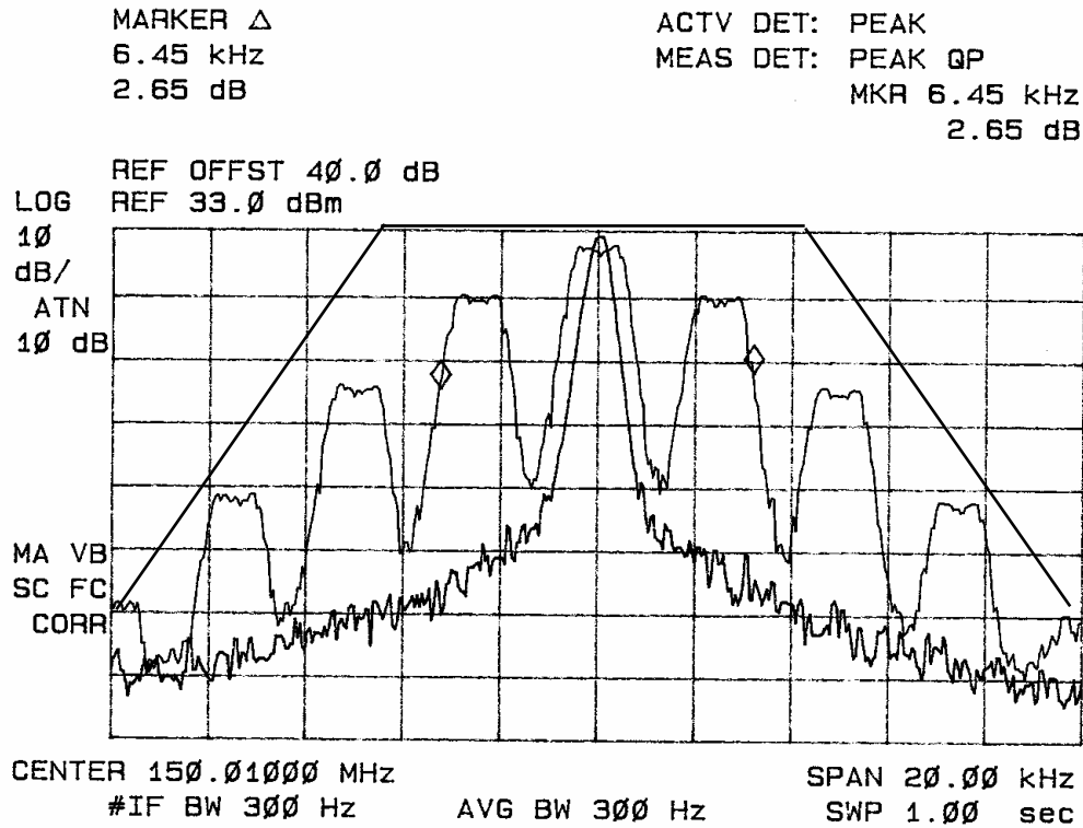
Figure nine Occupied Band Width, Narrow band, CTCSS
