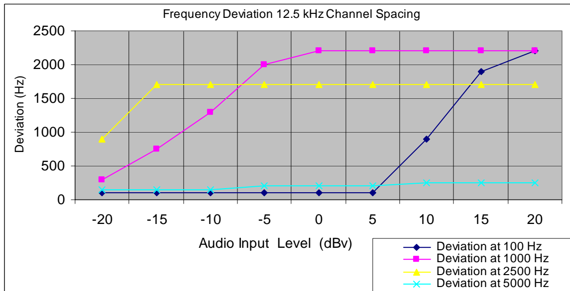
Figure three Frequency Deviation Characteristics (12.5 kHz Channel spacing)
