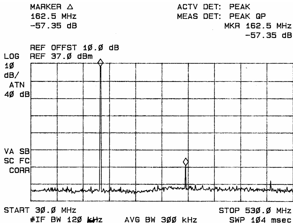
Figure eleven Emissions at Antenna Terminal (5 watt)
