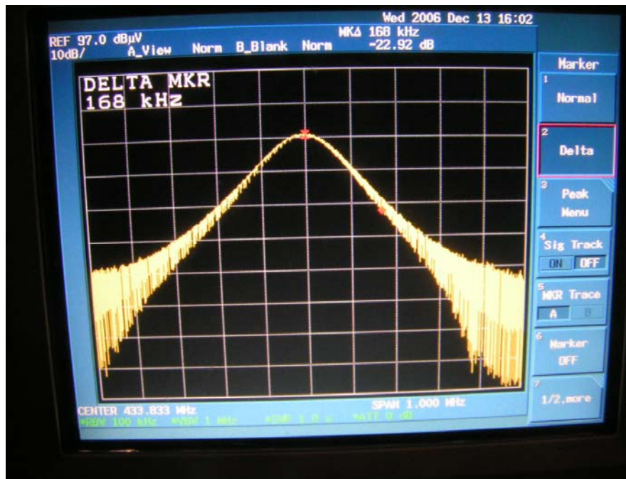
20dB Bandwidth #2
