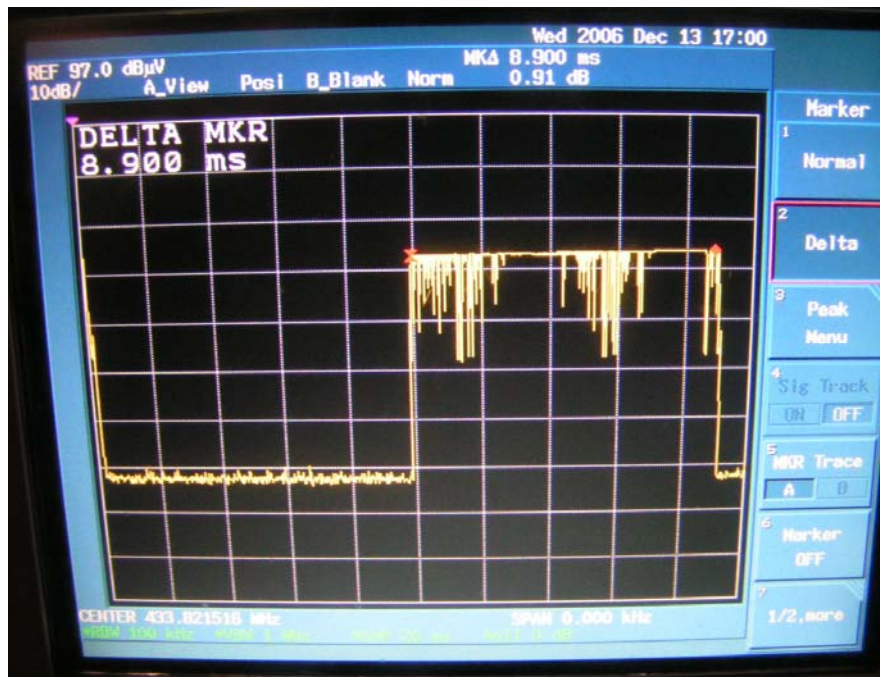
Transmission period
