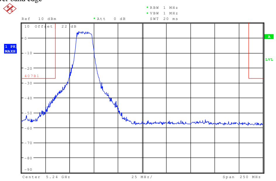
Plot 1: lower band edge
