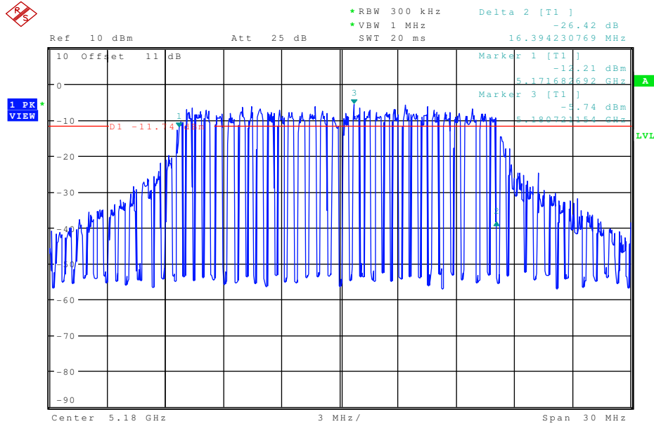
Plot 1: 5180 MHz 6 dB BW
