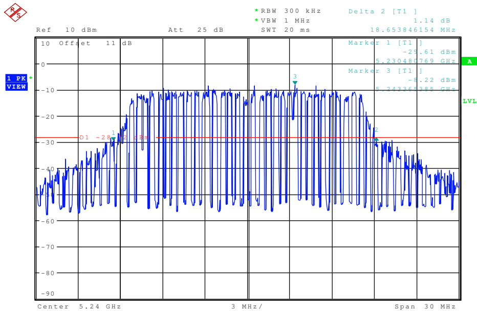
Plot 8: 5240 MHz 20 dB BW
