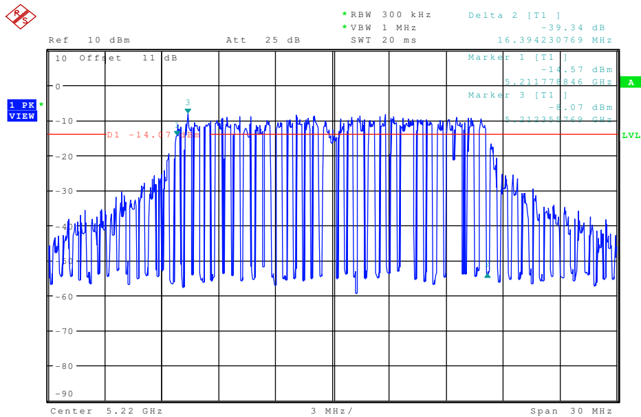
Plot 4: 5220 MHz 6 dB BW
