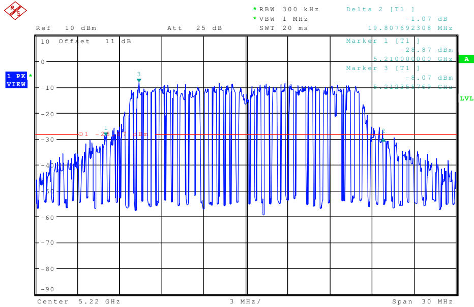
Plot 5: 5220 MHz 20 dB BW
