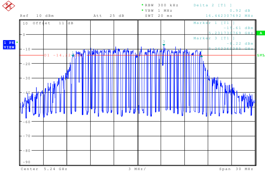
Plot 7: 5240 MHz 6 dB BW
