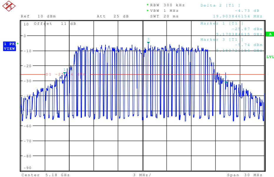
Plot 2: 5180 MHz 20 dB BW
