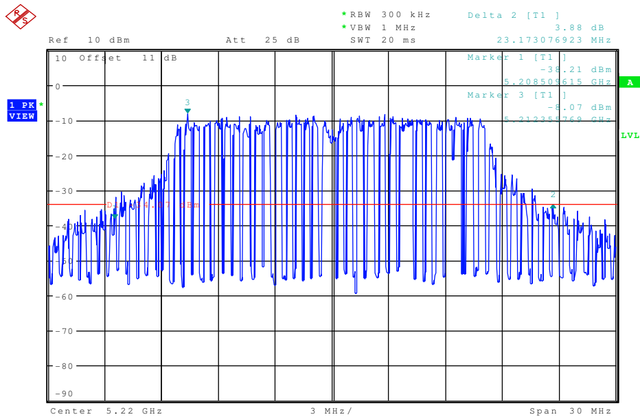
Plot 6: 5220 MHz 26 dB BW
