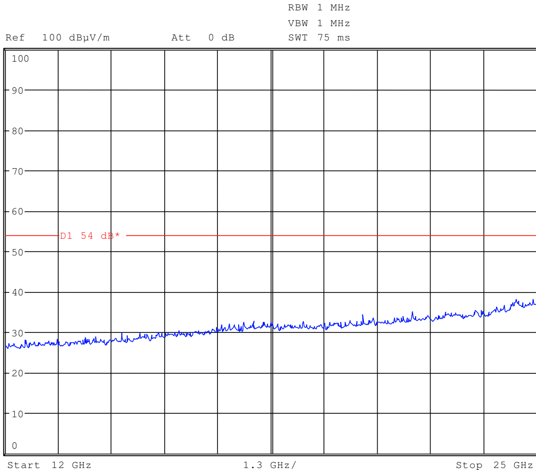
Plot 3: 12-25 GHz vertical (valid for all three channels) (worst case)
