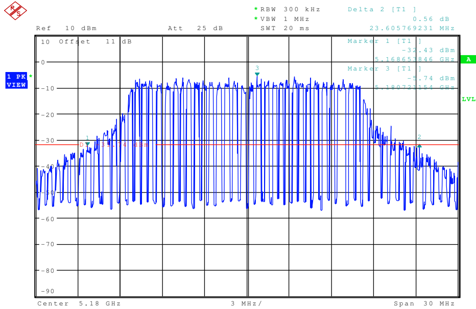
Plot 3: 5180 MHz 26 dB BW
