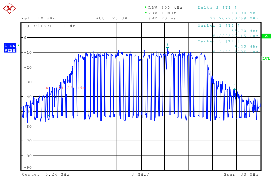
Plot 9: 5240 MHz 26 dB BW
