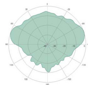
vertical 2450 MHz
