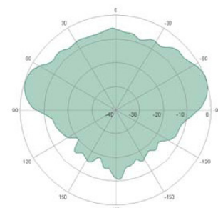
vertical 2450 MHz
