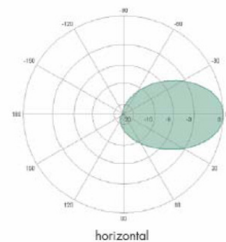
Radiation Pattern
