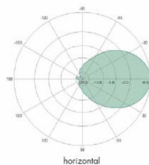
Radiation Pattern
