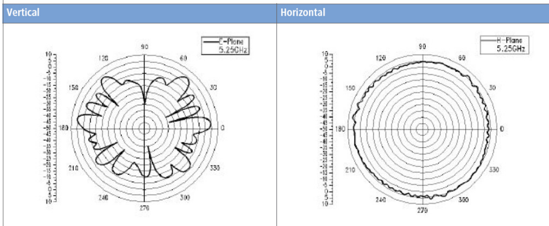
Directivity pattern 5.25GHz
