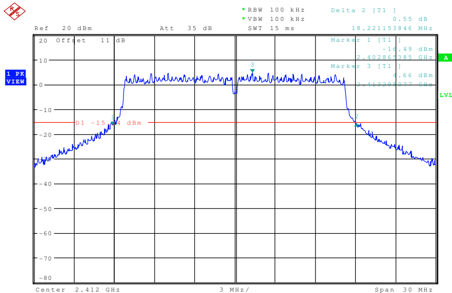
Plot 4: 20 dB-Bandwidth (2412 MHz)
