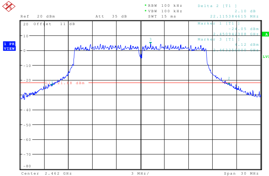
Plot 9: 26 dB-Bandwidth (2462 MHz)
