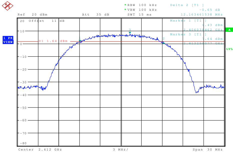
Plot 1: 6 dB-Bandwidth (2412 MHz)
