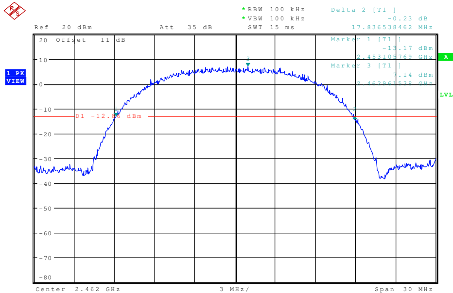
Plot 6: 20 dB-Bandwidth (2462 MHz)
