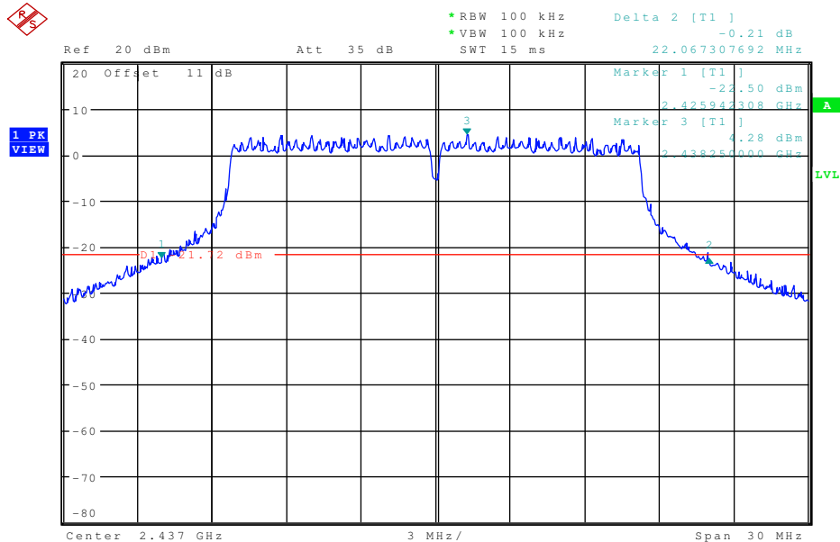
Plot 8: 26 dB-Bandwidth (2437 MHz)
