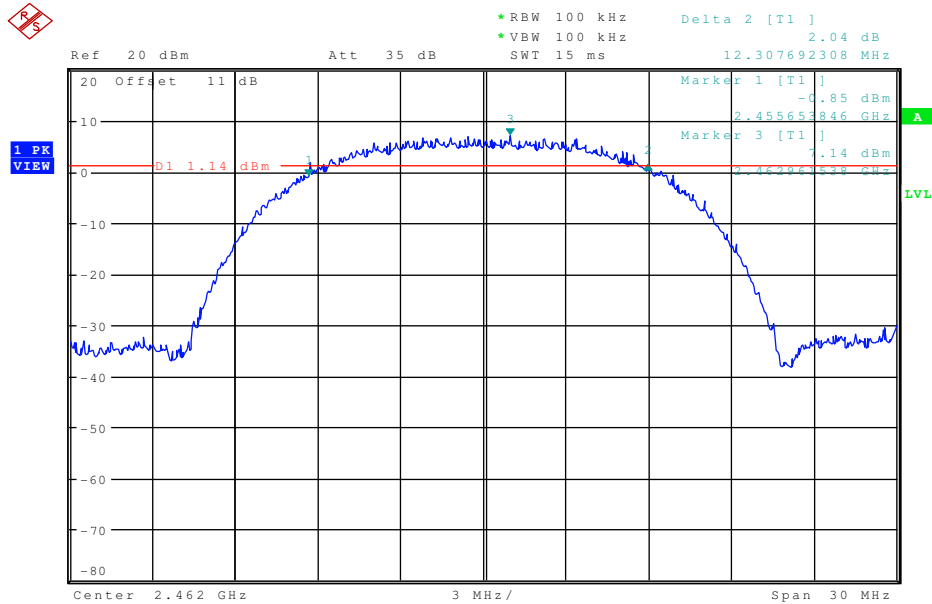
Plot 3: 6 dB-Bandwidth (2462 MHz)
