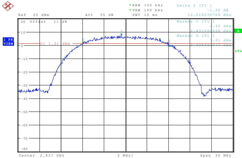
Plot 2: 6 dB-Bandwidth (2437 MHz)
