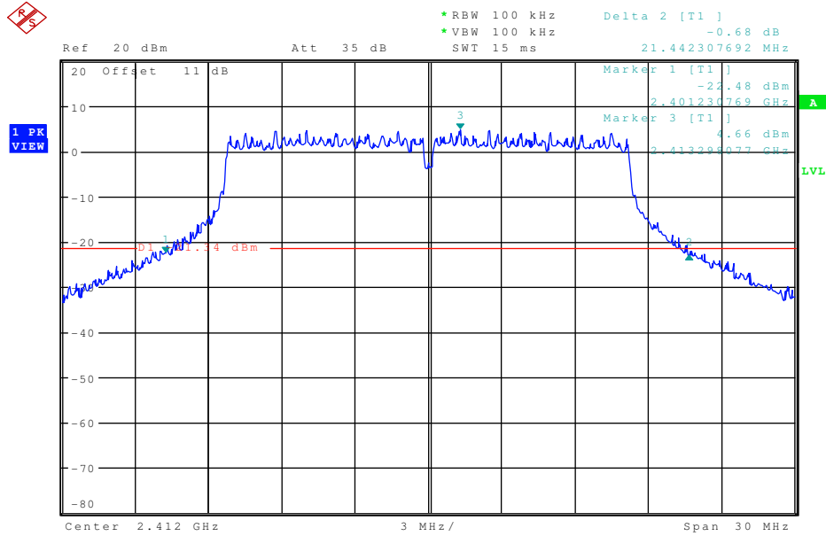
Plot 7: 26 dB-Bandwidth (2412 MHz)
