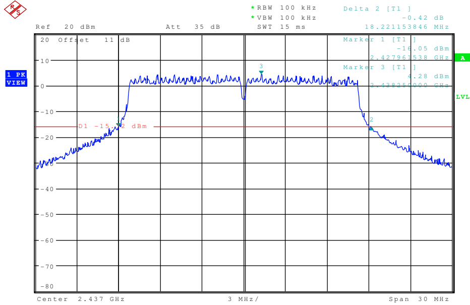
Plot 5: 20 dB-Bandwidth (2437 MHz)
