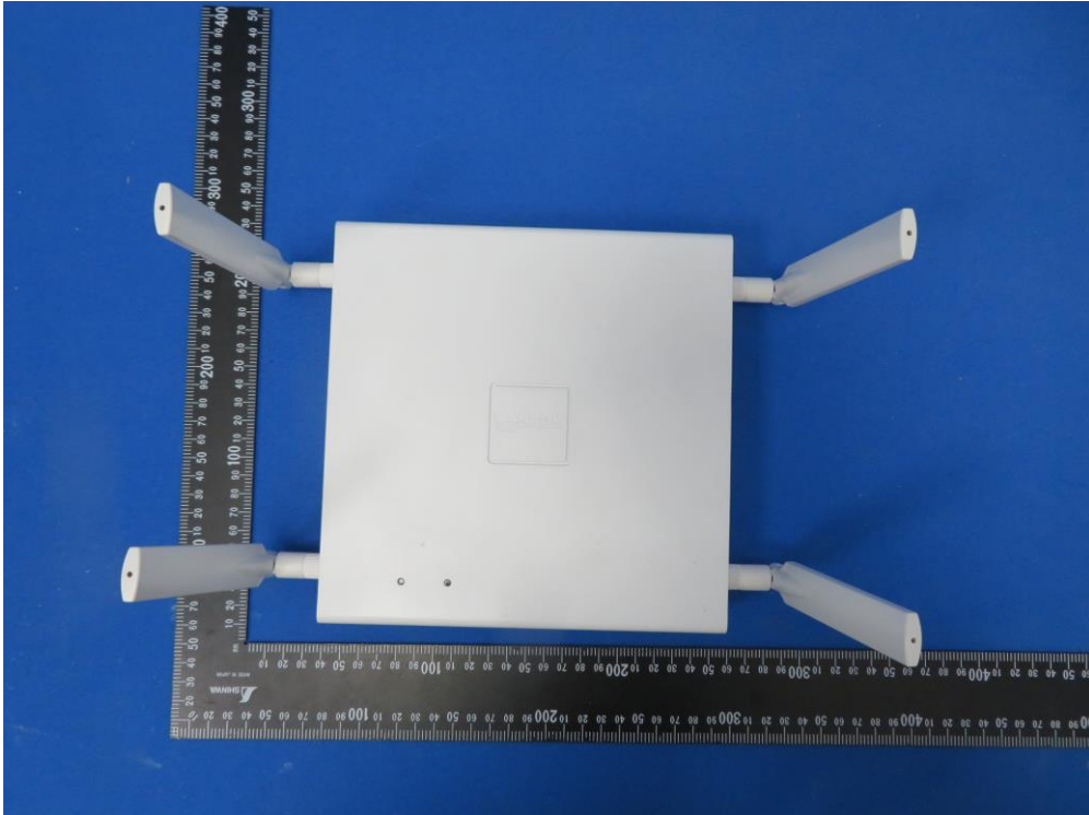
(7) EUT Photo (4x4 Indoor 11ax AP with External SMA Connector)
