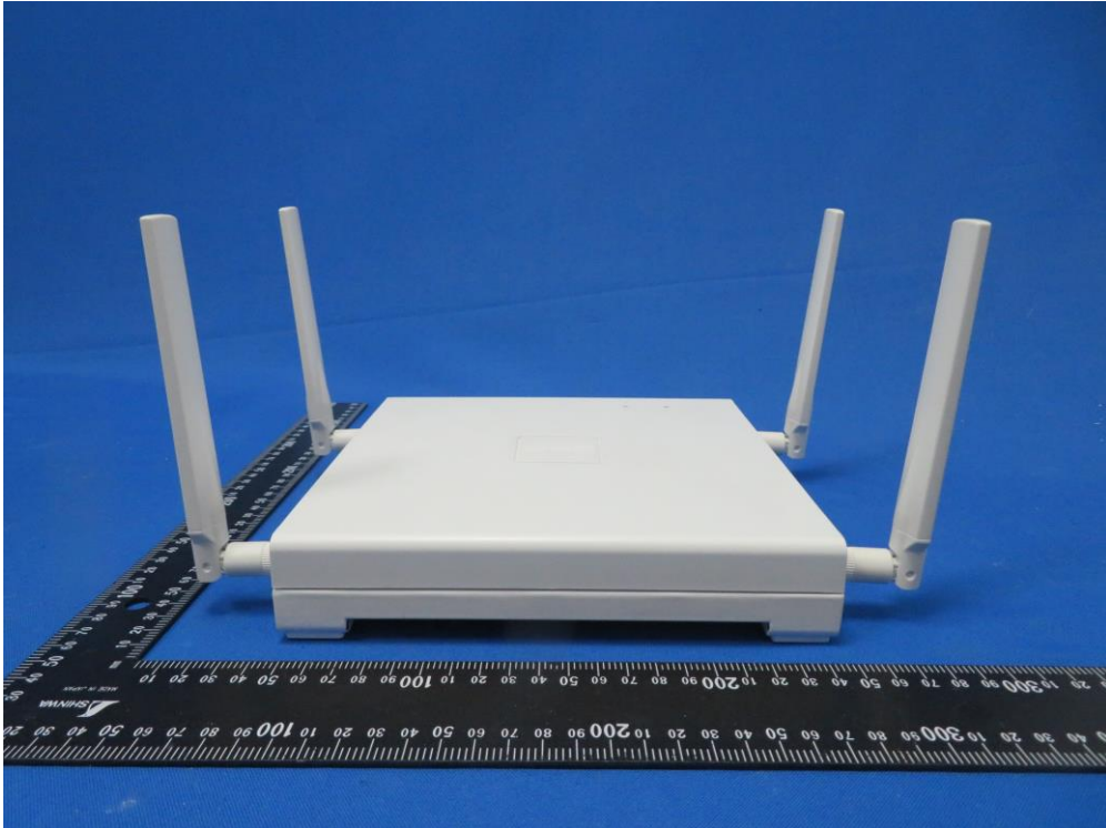
(11) EUT Photo (4x4 Indoor 11ax AP with External SMA Connector)
