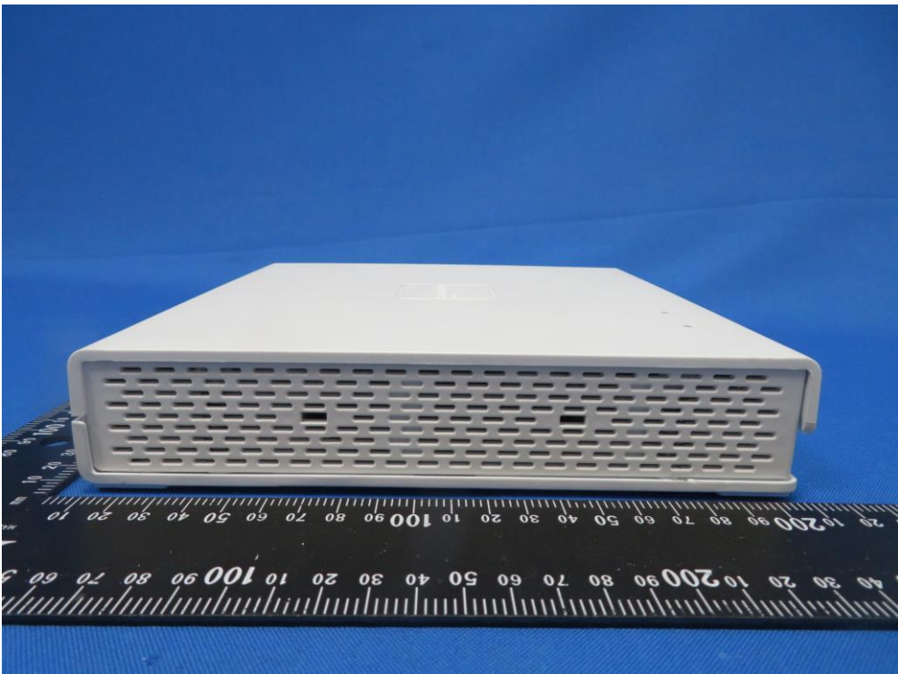
(6) EUT Photo (4x4 Indoor 11ax AP with Internal Antenna)
