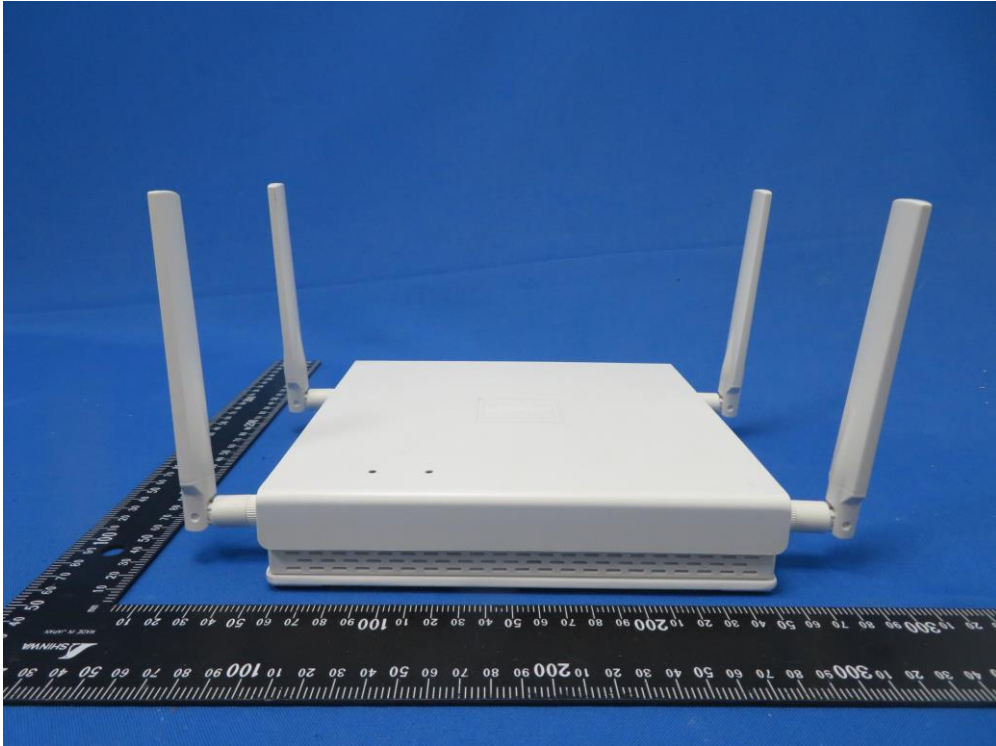
(9) EUT Photo (4x4 Indoor 11ax AP with External SMA Connector)
