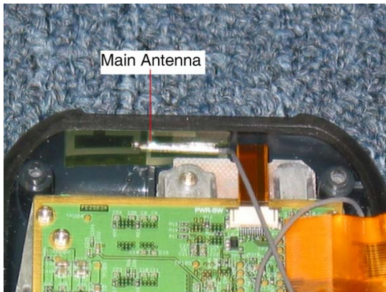
Main Antenna
