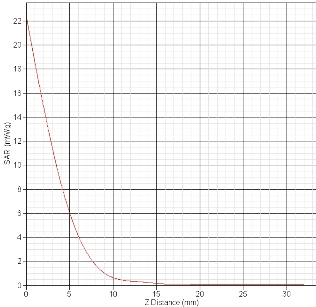
SAR-Z Axis at Hotspot x:0.31 y:-0.19
