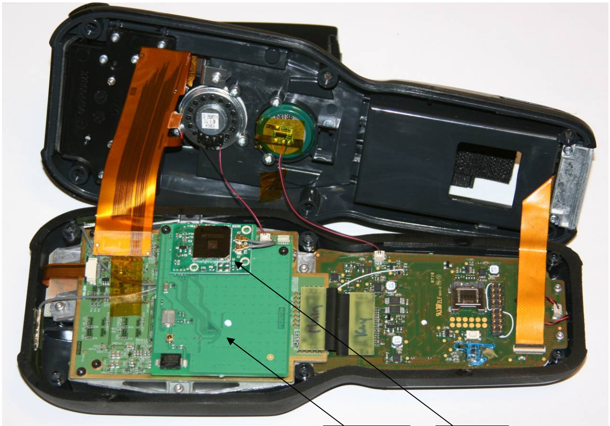
Falcon X3 – Opened showing location of Bluetooth board and WiFi Module (Detailed photographs of top/bottom sides of the radios are provided in separate files)
