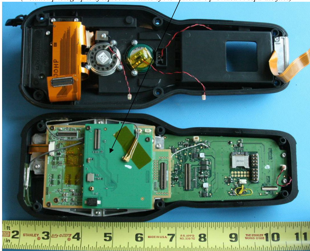
Falcon X3 – Opened showing location of Bluetooth board and WiFi Module (Detailed photographs of top/bottom sides of the radios are provided in separate files)
