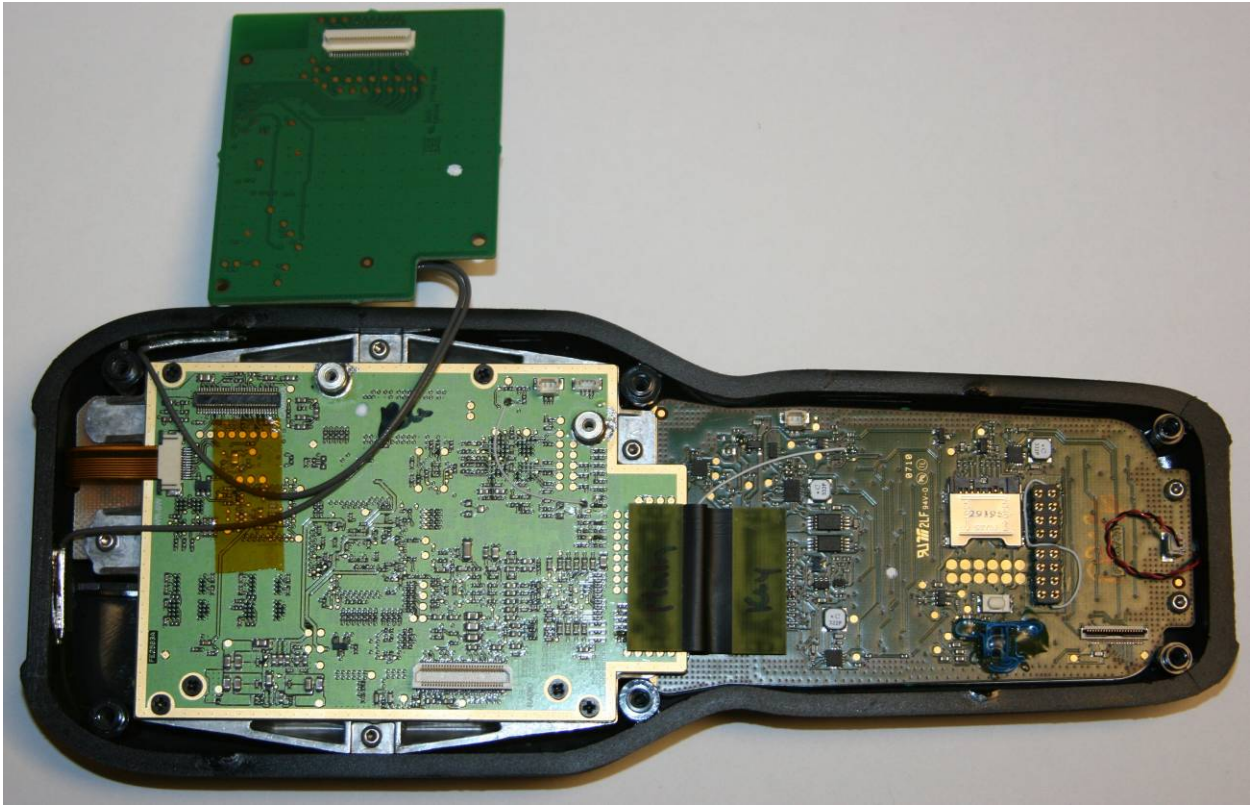
Opened, Bluetooth card removed
