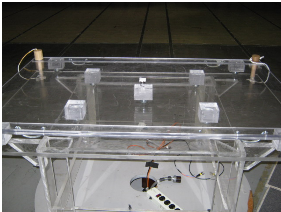
Back View - Radiated Emissions (Spurious below 12 GHz.)
