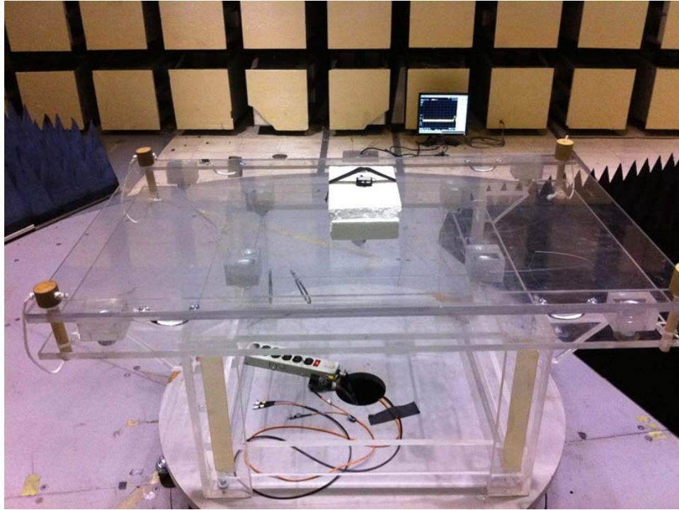
Radiated Emissions – Power (Flat position.)
