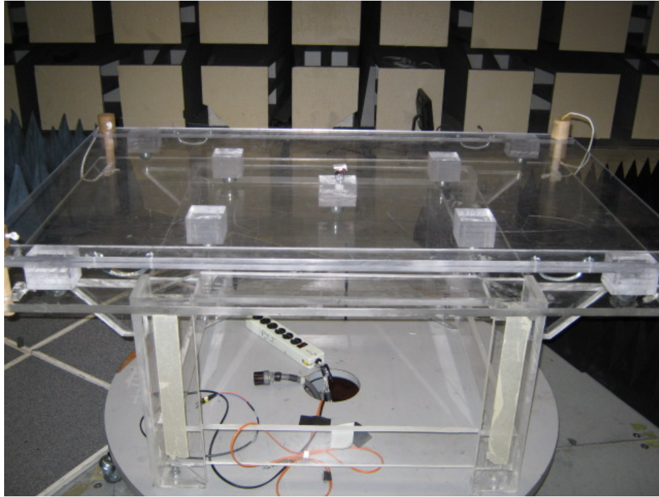
Front View - Radiated Emissions (Spurious below 12 GHz.)
