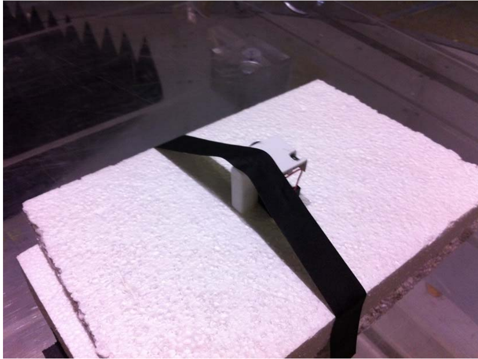
Radiated Emissions – Power (Side position.)
