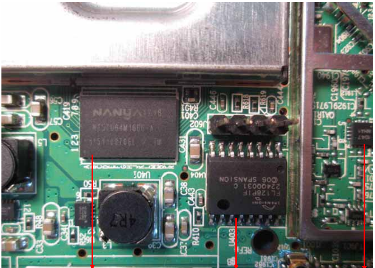
DDR2 NT5TU64M16GG-AC
