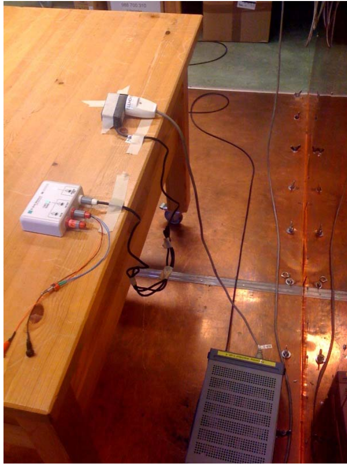
Conducted emission
