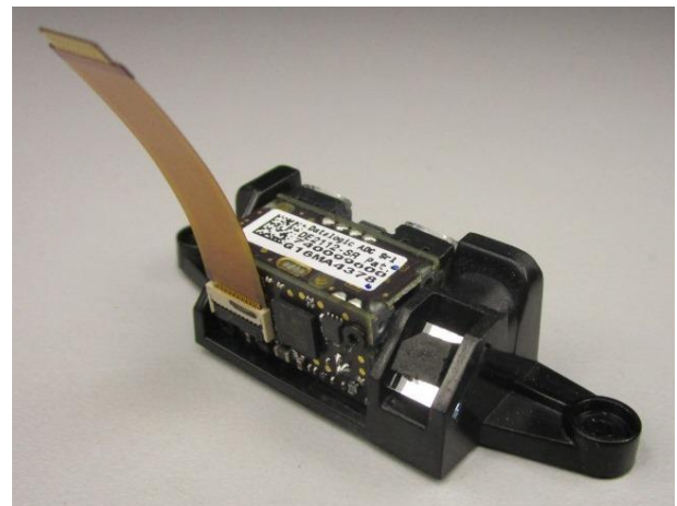
2D Imager with plastic support and Green Spot
