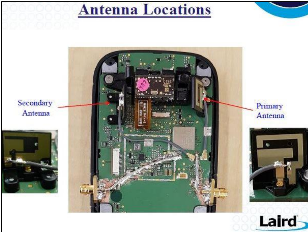
Photo 32: Antenna Locations
